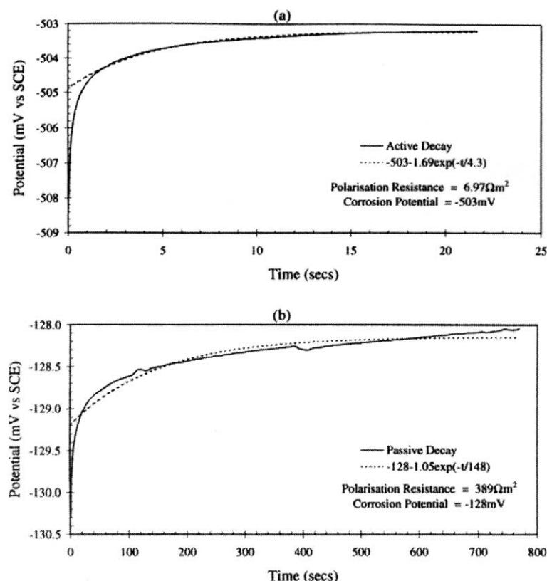
Fig. 9. Slow coulостatic transient obtained on (a) active and (b) passive steel in concrete. The potential decay shown represents 90% of the potential shift at 1 s (Note the different \times scales). From Ref. [73].
