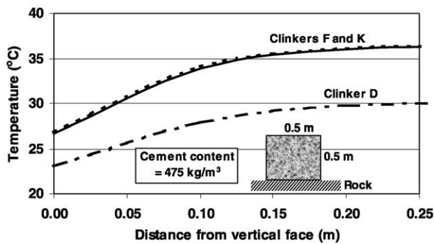
Fig. 7. Modelled temperatures across a central section of a concrete beam at the time when the maximum temperature occurs, for the three cement heat rates assessed.
