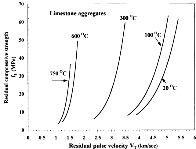
Fig. 17. Relation between pulse velocity and residual compressive strength after heating at various temperatures. Limestone concretes.
