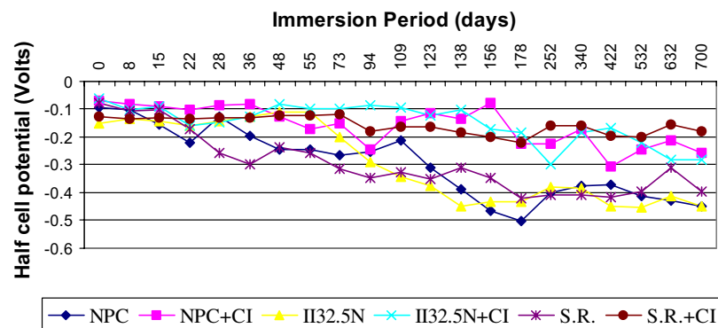
Fig. 2. Half cell potential measurements of NPC, SR and II32.5N mortars with and without corrosion inhibitor (CI) immersed in 5% NaCl solution for 2 years.
