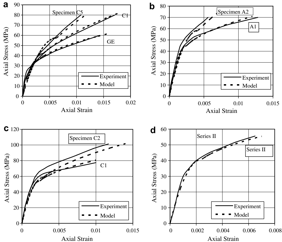
Fig. 4. Comparison of model prediction with experimental results for circular columns (from Hantouche and Harajli [20]): (a) Toutanji [8], (b) Nanni et al. [18], (c) Miyauchi et al. [19], (d) Teng and Lam [15].
