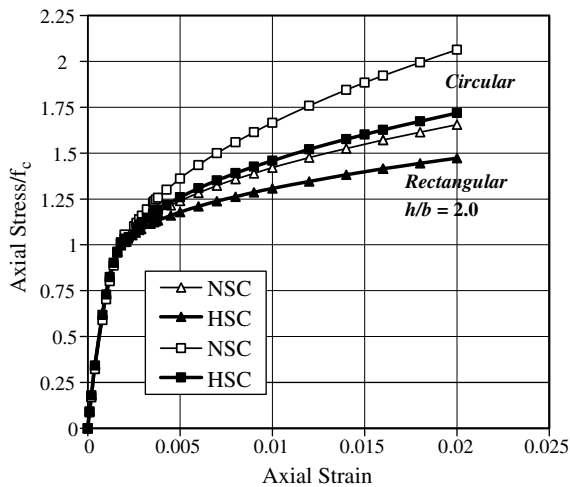
Fig. 10. Effect of f'_c on FRP confinement effectiveness in increasing the axial strength.
