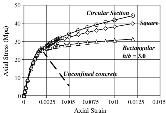
Fig. 8. Effect of section type on the predicted stress–strain response.
