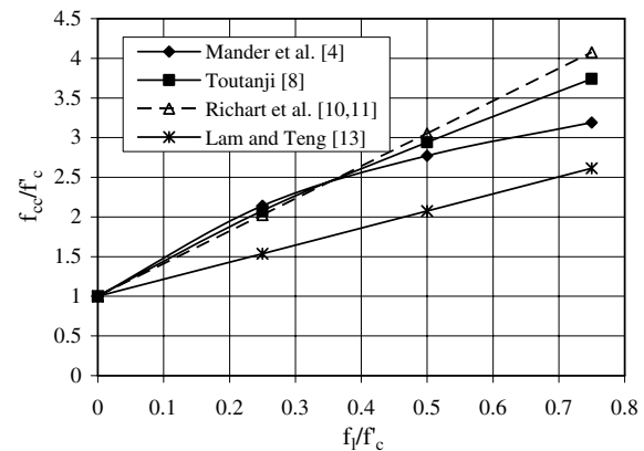
Fig. 1. Variation of confinement effectiveness with confinement ratio.
