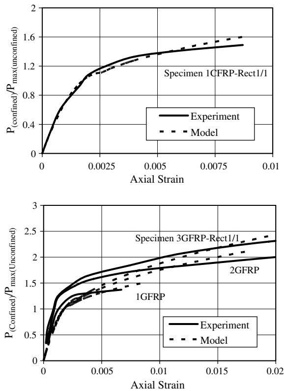
Fig. 6. Comparison of analytical predictions with the test data of Cole and Belarbi [21].
