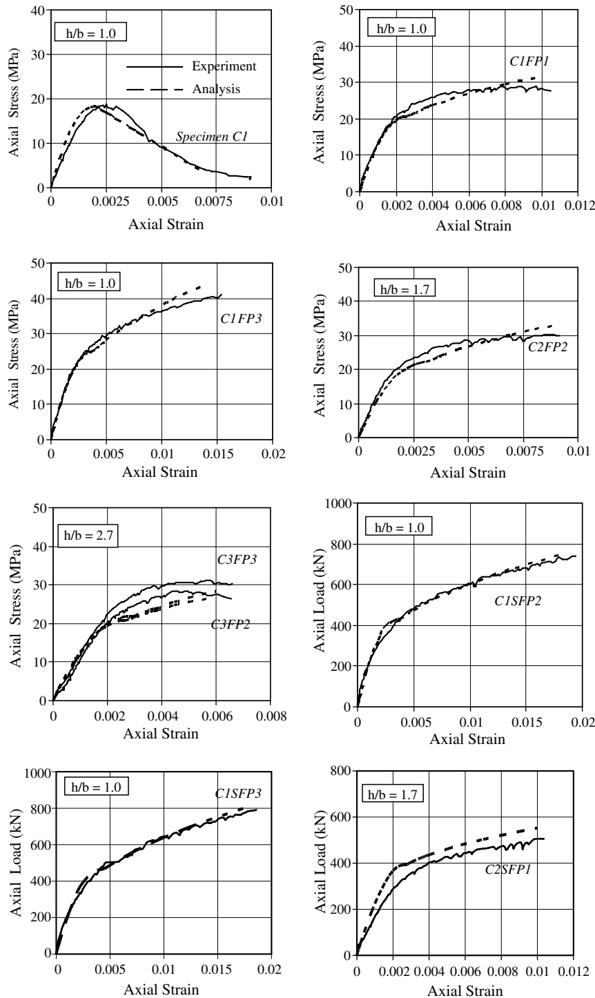
Fig. 5. Comparison of analytical predictions with the experimental results of rectangular columns of Hantouche and Harajli [20].
