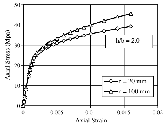
Fig. 9. Effect of corner radius on the predicted stress–strain response.
