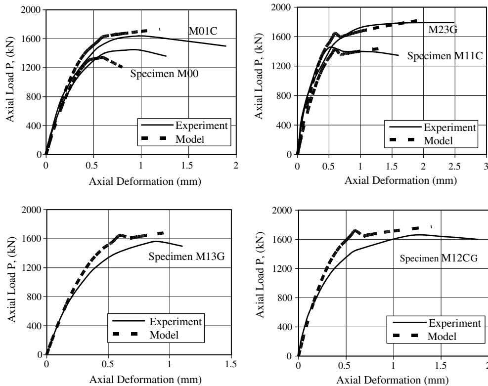
Fig. 7. Comparison of model prediction with the test data of Tan [5].
