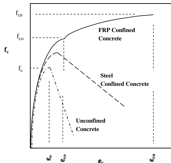
Fig. 2. Proposed stress–strain relationship for FRP confined concrete.
