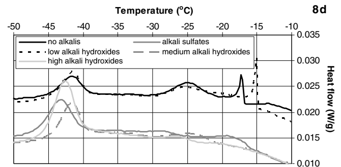
Fig. 4. LTC results for CCRL 140 w/c = 0.40 cement pastes with and without alkali additions cured under saturated conditions for 8 d.
