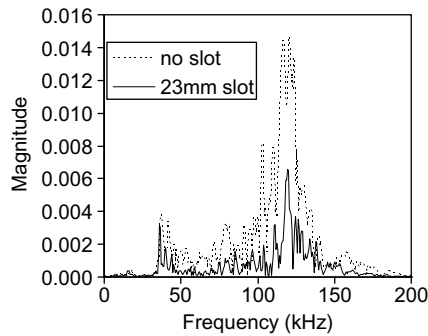
Fig. 5. Fast Fourier transform of different signals.
