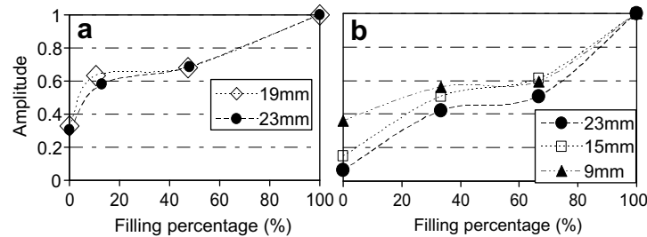
Fig. 8. Amplitude vs. epoxy filling percentage of different slots: (a) experimental, and (b) numerical results (curves connecting the symbols indicate basic trends and are not results of curve fitting).
