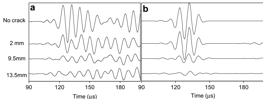
Fig. 2. Waveforms collected after different slots, using excitation of 115 kHz: (a) experimental, and (b) numerical results.
