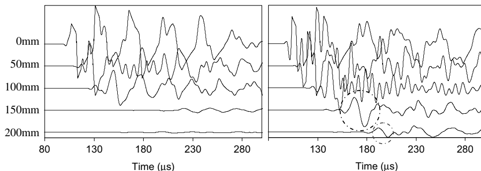
Fig. 10. Waveforms collected at different distances from the excitation on the bridge deck: (a) before and (b) after repair with epoxy injection. The crack is at the position of 125 mm.
