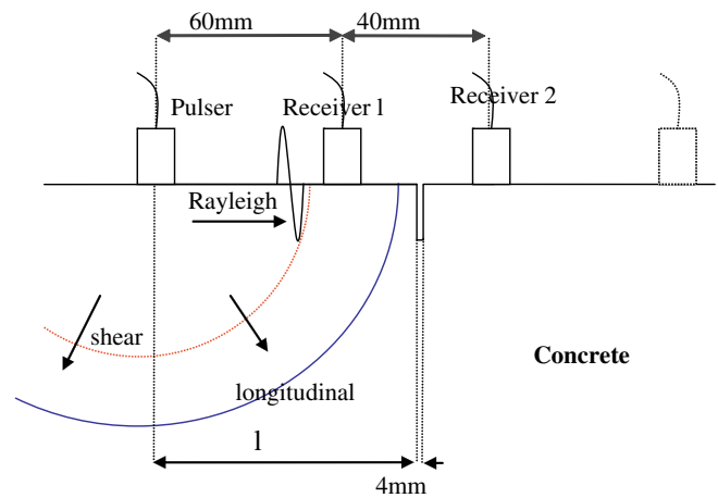
Fig. 1. Geometry of the experiment.
