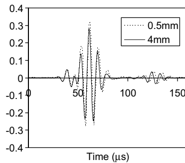
Fig. 9. Waveforms of 115 kHz collected after 9.5 mm deep slot for different slot width.
