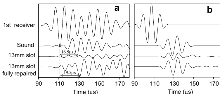
Fig. 6. Waveforms collected for different conditions of concrete: (a) experimental, and (b) numerical results.
