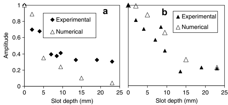
Fig. 3. Amplitude vs. slot depth relationship using: (a) 115 kHz and (b) 50 kHz.
