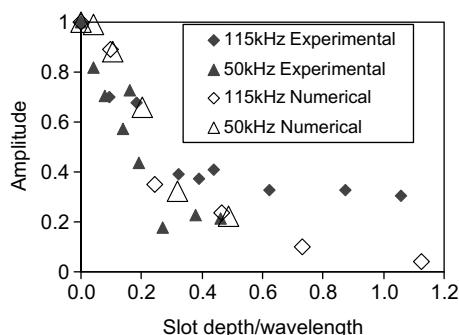
Fig. 4. Amplitude vs. slot depth/wavelength relationship.
