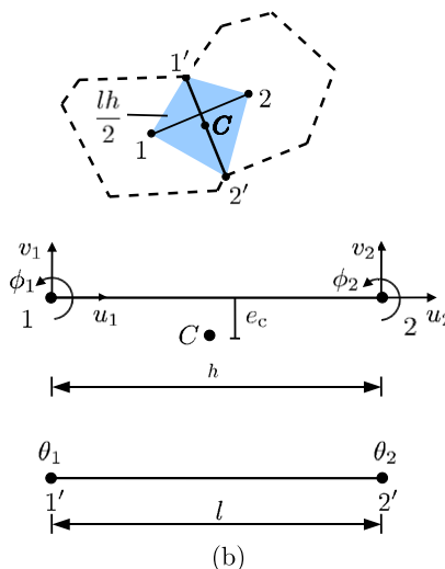
Fig. 1. Discretisation: (a) Elements (solid lines) and corresponding cross-sections (dashed lines) of the mechanical lattice obtained from the Delaunay triangulation and dual Voronoi tessellation, respectively. (b) Degrees of freedoms of the lattice elements for the mechanical and transport model in the local co-ordinate system.
