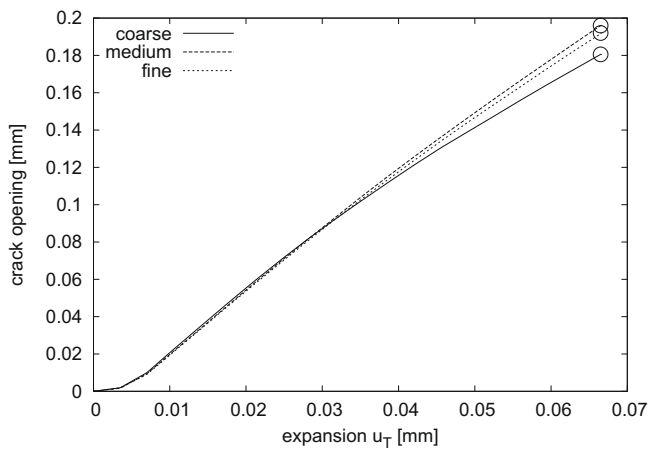
Fig. 10. Results of the structural analysis: Crack-opening versus eigen-displacement u_T for three mesh-sizes. The open circles mark stages at which the flow analysis is performed.
