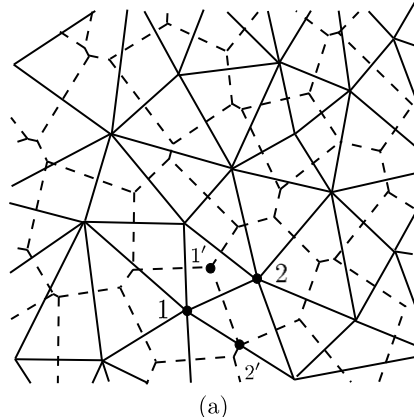
Fig. 1. Discretisation: (a) Elements (solid lines) and corresponding cross-sections (dashed lines) of the mechanical lattice obtained from the Delaunay triangulation and dual Voronoi tessellation, respectively. (b) Degrees of freedoms of the lattice elements for the mechanical and transport model in the local co-ordinate system.
