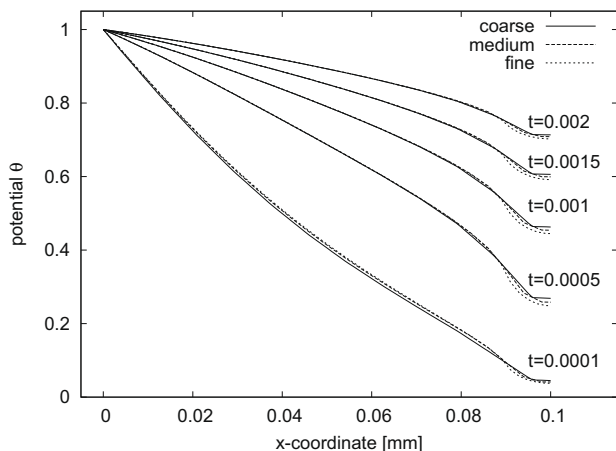
Fig. 7. Potential in x -direction along the crack at y = 0.05 m for several time steps.
