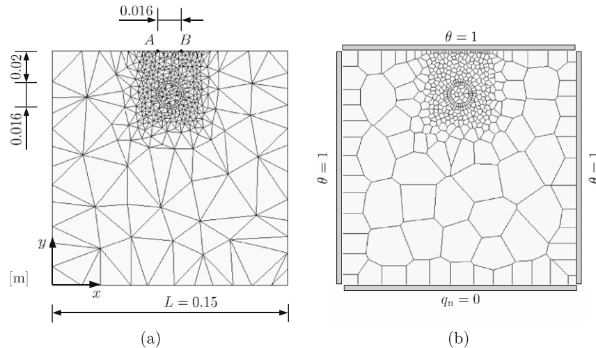
Fig. 9. Random lattices with inclusions for (a) structural and (b) transport analysis for d_m = 0.002 m in the refined regions of the specimens.
