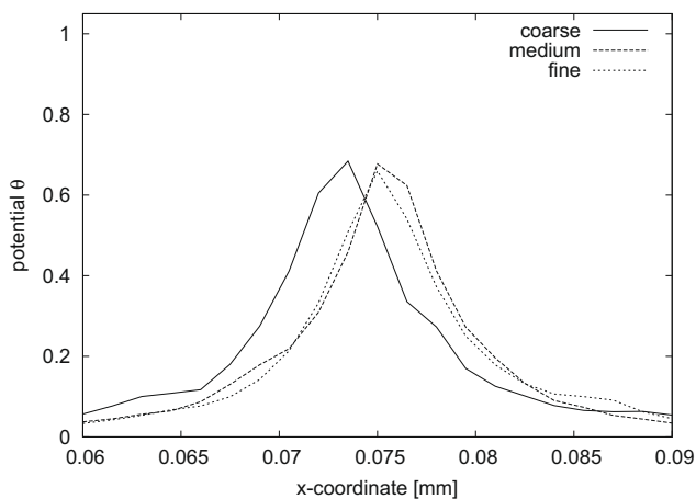
Fig. 11. Results of the flow analysis: Potential \theta along the x -direction ( y = 0.135 m) in the refined region of the mesh for three element sizes at a eigen-displacement of u_T = 0.0665 mm and t = 0.00001 s.
