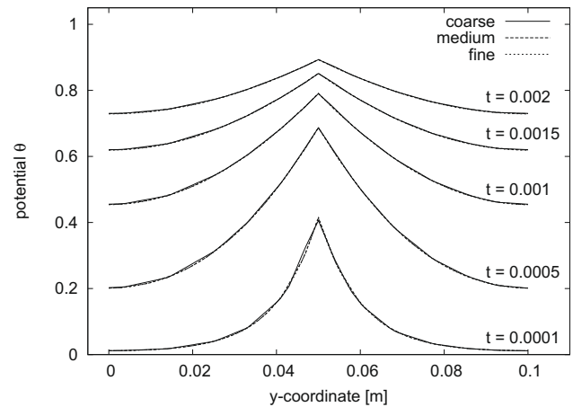
Fig. 8. Potential in y -direction perpendicular to the crack at x = 0.05 m for several time steps.
