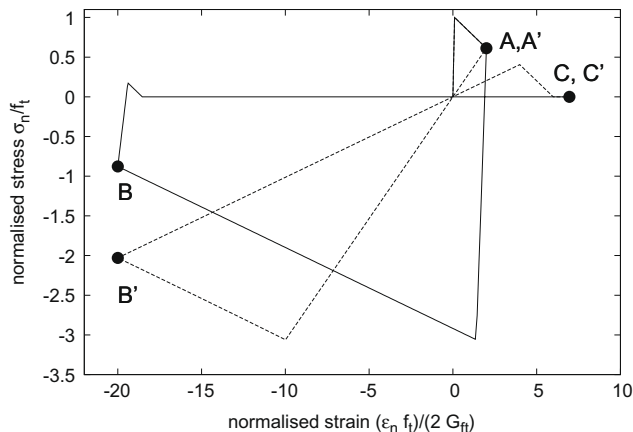
Fig. 2. Stress–strain response for fluctuating normal strains for \mu = 1 (solid line) and \mu = 0 (dashed line).
