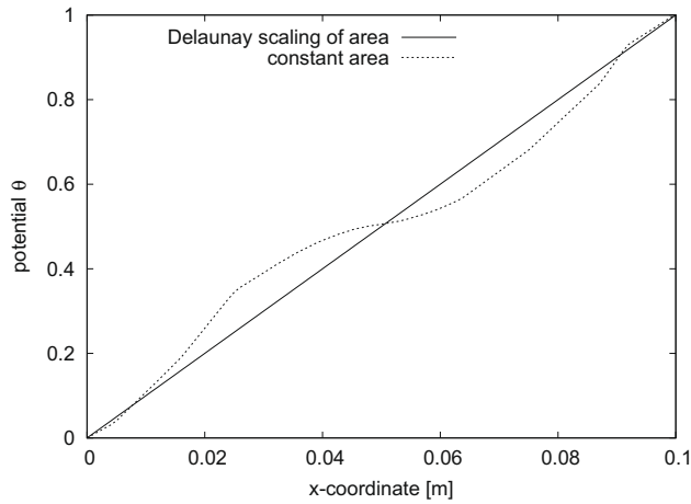
Fig. 4. Comparison of the potential \theta along the x -direction ( y = L/2 ) for cross-sections obtained with the Delaunay triangulation and a constant average cross-section.
