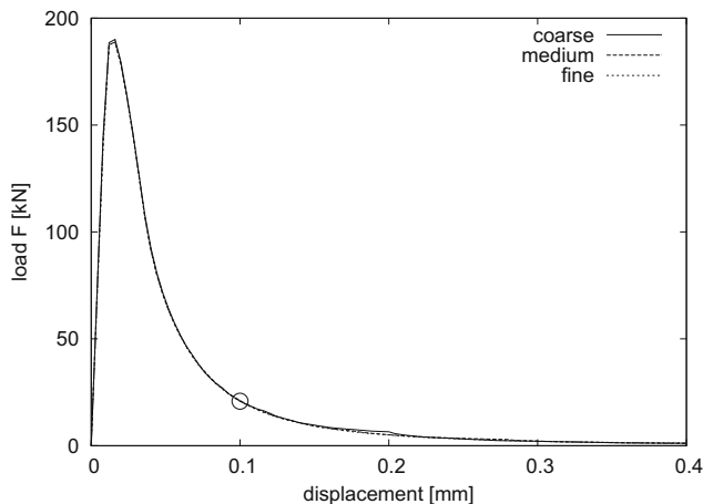
Fig. 6. Results of the structural analysis: load–displacement curves for three element sizes. The open circle marks the stage for which the flow analyses are performed in the second stage of the analysis.
