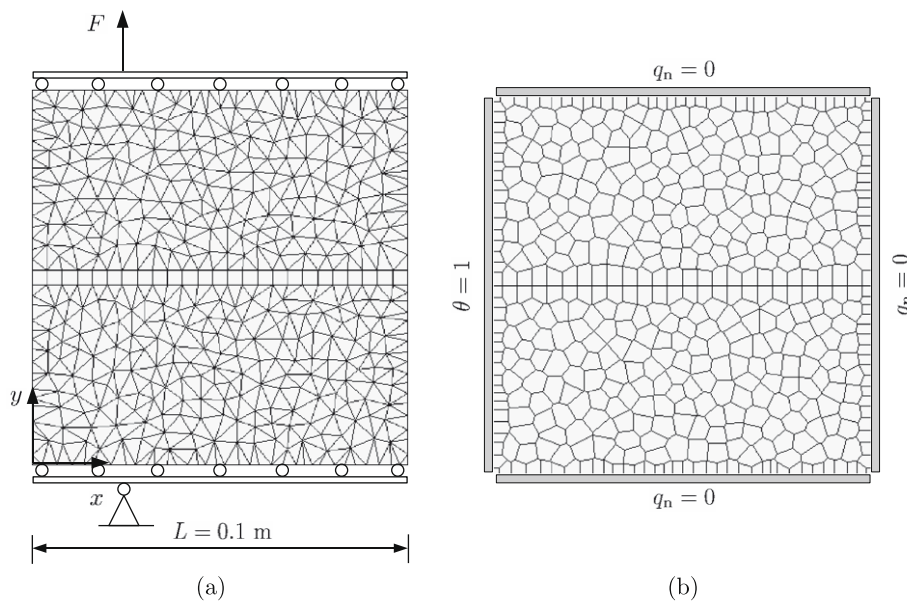
Fig. 5. Meshes and loading set-up for (a) structural and (b) transport analysis for the medium density lattice with elements aligned along the potential crack path.
