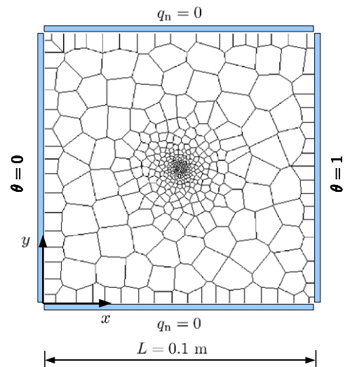
Fig. 3. Discretisation of the domain by means of a graded network. Lattice elements are located on the facets of the Voronoi polygons.
