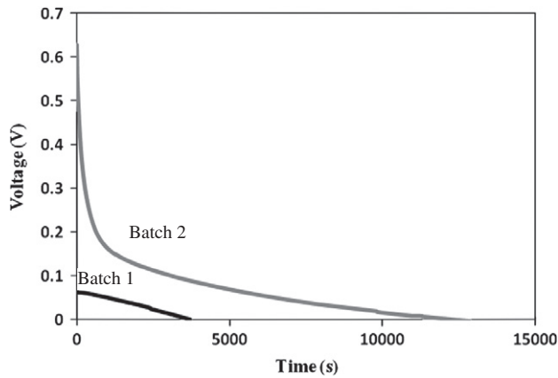
Fig. 6. Constant-current discharge at 60 \mu\text{A} for Battery 2 at 28 days curing. Batch 1: \rho_1 = 9375 \Omega\text{ cm} ; \rho_2 = 11,718 \Omega\text{ cm} ; V_{oc} = 0.22\text{ V} ; f = 1.6 \times 10^{-5} ; Batch 2: \rho_1 = 1631 \Omega\text{ cm} ; \rho_2 = 1931 \Omega\text{ cm} ; V_{oc} = 0.72\text{ V} ; f = 5.2 \times 10^{-5} .
