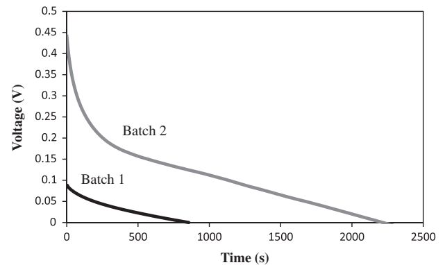
Fig. 8. Constant-current discharge at 100 \mu\text{A} for Battery 2 at 28 days of curing. Batch 1: \rho_1 = 3766 \Omega\text{ cm} ; \rho_2 = 4384 \Omega\text{ cm} ; V_{oc} = 0.21\text{ V} ; f = 2.2 \times 10^{-6} ; Batch 2: \rho_1 = 1687 \Omega\text{ cm} ; \rho_2 = 2053 \Omega\text{ cm} ; V_{oc} = 0.64\text{ V} ; f = 1.6 \times 10^{-5} .
