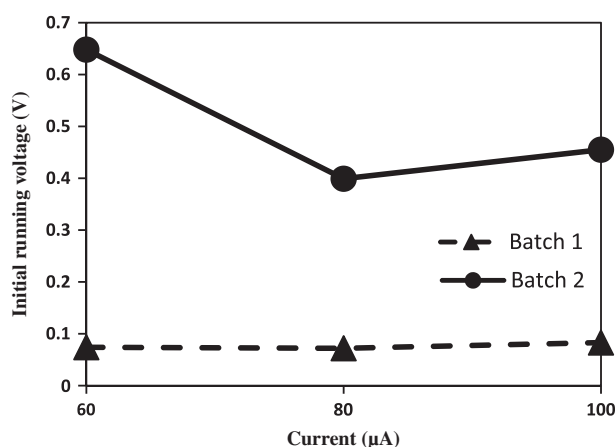
Fig. 11. Cement-based battery initial running voltage vs. discharge current for Battery 2.
