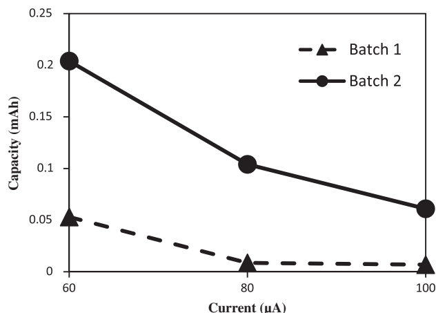
Fig. 10. Cement-based battery capacity vs. discharge current for Battery 2.
