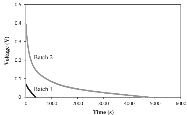
Fig. 7. Constant-current discharge at 80 \mu\text{A} for Battery 2 at 28 days of curing. Batch 1: \rho_1 = 2590 \Omega\text{ cm} ; \rho_2 = 3640 \Omega\text{ cm} ; V_{oc} = 0.21\text{ V} ; f = 2.2 \times 10^{-6} ; Batch 2: \rho_1 = 1922 \Omega\text{ cm} ; \rho_2 = 2309 \Omega\text{ cm} ; V_{oc} = 0.62\text{ V} ; f = 2.7 \times 10^{-5} .
