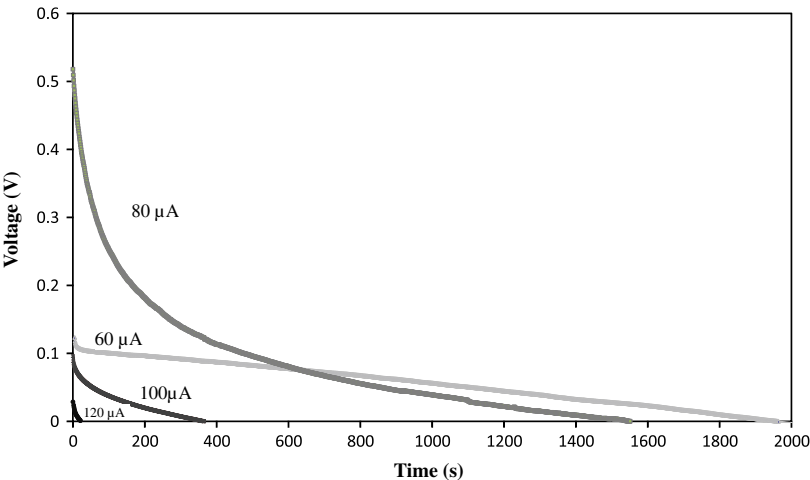
Fig. 5. Constant-current discharge of Battery 2 at 7 days curing. Battery at 60 \mu\text{A} : \rho_1 = 5376 \Omega \text{ cm} ; \rho_2 = 10,752 \Omega \text{ cm} ; V_{oc} = 0.21 \text{ V} ; f = 2.1 \times 10^{-6} ; Battery at 80 \mu\text{A} : \rho_1 = 4860 \Omega \text{ cm} ; \rho_2 = 8640 \Omega \text{ cm} ; V_{oc} = 0.23 \text{ V} ; f = 2.2 \times 10^{-6} ; Battery at 100 \mu\text{A} : \rho_1 = 4320 \Omega \text{ cm} ; \rho_2 = 10,800 \Omega \text{ cm} ; V_{oc} = 0.18 \text{ V} ; f = 1.1 \times 10^{-5} ; Battery at 120 \mu\text{A} : \rho_1 = 3430 \Omega \text{ cm} ; \rho_2 = 9384 \Omega \text{ cm} ; V_{oc} = 0.19 \text{ V} ; f = 1.9 \times 10^{-7} .
