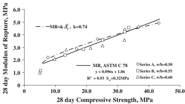
Fig. 12. Modulus of rupture vs. compressive strength at 28 d for series A, B, and C, and curve for the equation MR = k \sqrt{f_c} with k = 0.74 . S_{yx} indicates standard error from linear regression.
