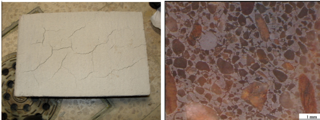
Fig. 5. Mortar prepared with quicklime pieces, QM.1-7 (7-day maturation).
