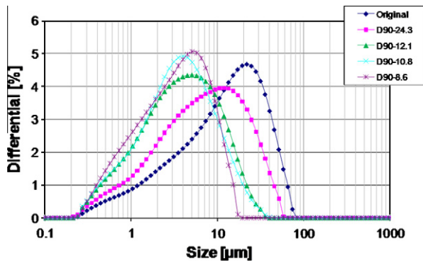
Fig. 1. Particle size distributions of the five cements shown as probability density functions. Each curve is the average of six individual measurements and the error bars (one standard deviation) would fall within the size of the shown symbols.
