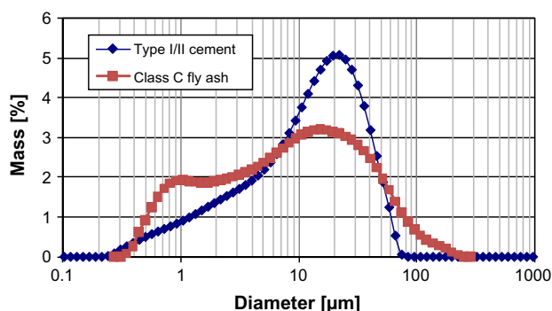
Fig. 1. Measured particle size distributions for the cement and fly ash investigated in the study. Results are the average of six individual measurements and error bars (one standard deviation) would fall within the size of the symbols.
