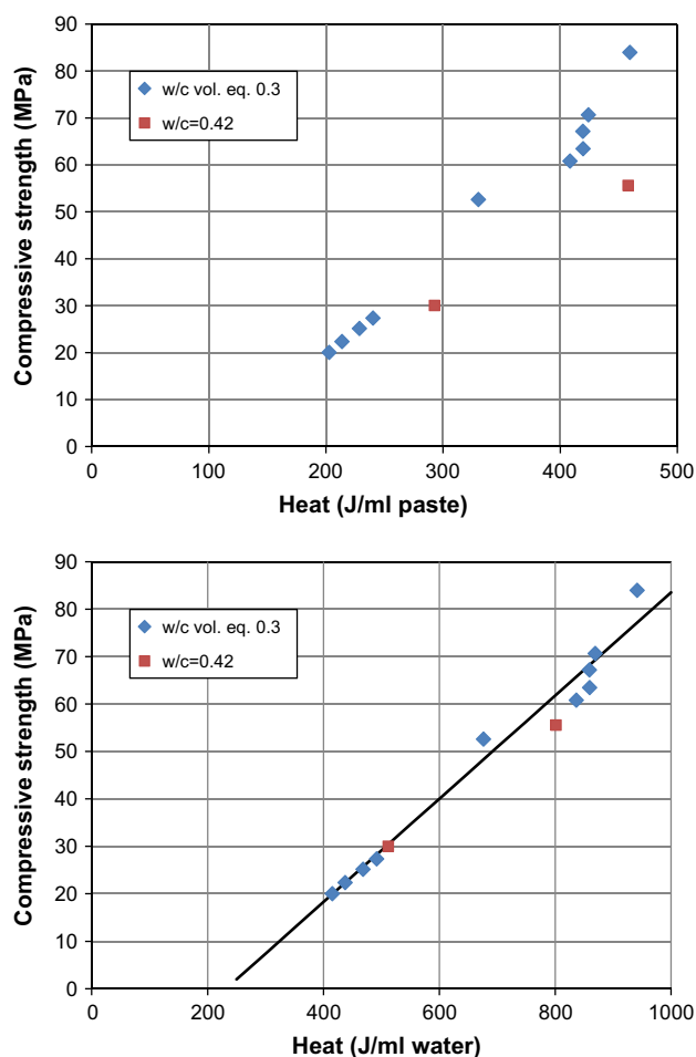
Fig. 9. Measured compressive strengths vs. measured cumulative heat release on either a per milliliter paste basis (top) or a per milliliter initial water basis (bottom) for mortars at ages of 1 d and 7 d.
