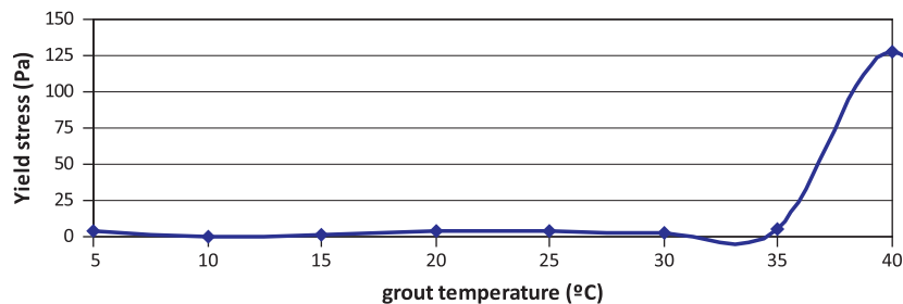
Fig. 22. Yield stress values of CEMI 42.5R + SF = 2% + HRWR = 0.5% with w/b = 0.30.
