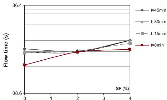
Fig. 9. Flow time for 0, 15, 30 and 45 min of resting time, after grout preparation, for different SF dosages tested (% of binder mass) and for a HRWR = 0.5%.
