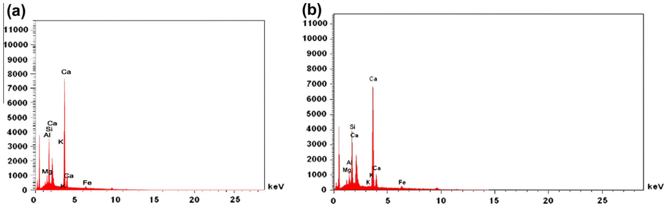
Fig. 16. Cement grout EDS spectrum at 365 d: (a) SF = 0% and (b) SF = 2%.
