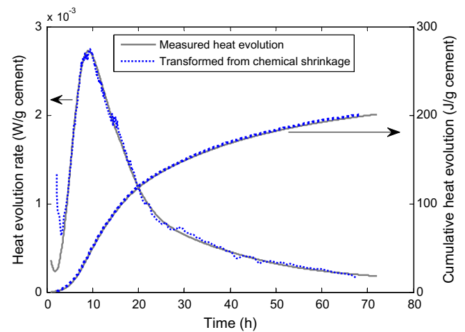
Fig. 6. Heat evolution curves vs. transformed chemical shrinkage curves (Class H-P cement, w/c = 0.38 , 25 °C).
