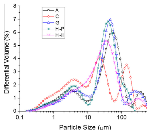
Fig. 1. Particle size distributions of different classes of cements.
