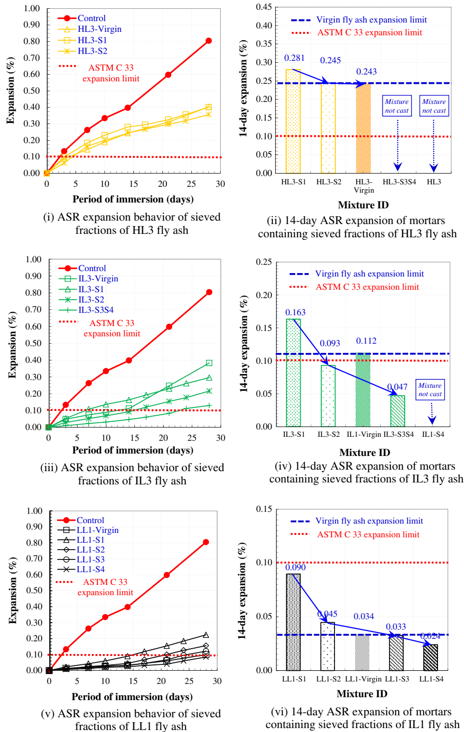
Fig. 5. ASR expansion behavior of mortars containing sieved fly ash fraction at a constant fly ash replacement level of 25%.
