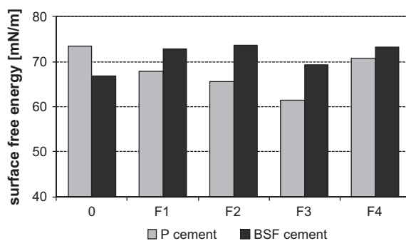
Fig. 4. Comparison of surface free energy of slurries.
