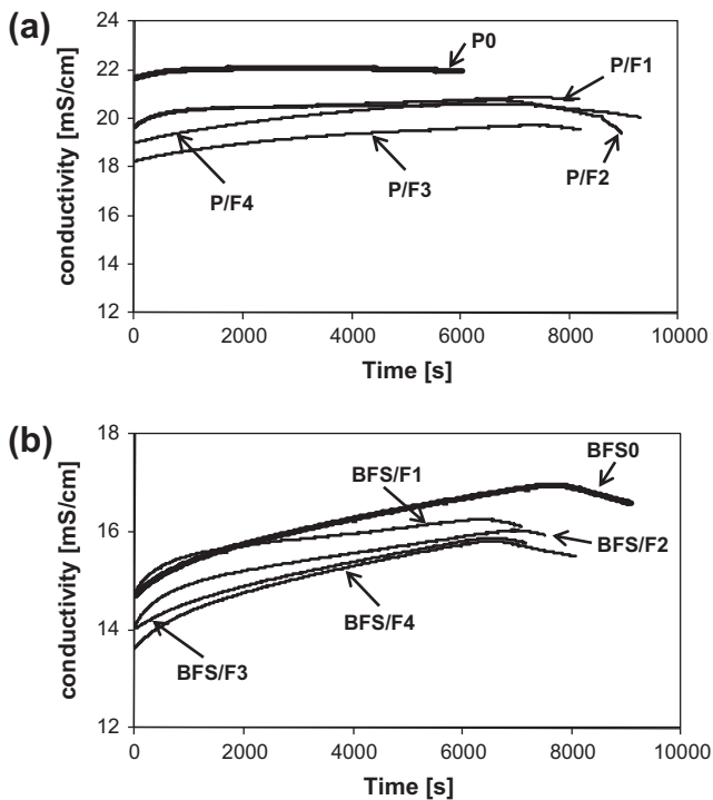
Fig. 7. Conductivity of Portland cement slurries (a) and BFS cement-based slurries (b) modified by limestone fillers.
