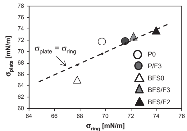
Fig. 6. Correlation between value of surface free energy of liquids measured with Ring method ( \sigma_{\text{ring}} ) and Wilhelmy plate method ( \sigma_{\text{plate}} ).
