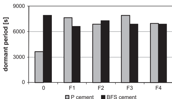
Fig. 8. Comparison of the initial time of the dormant period for Portland (P) and blast furnace slag (BFS)-based cement slurries.
