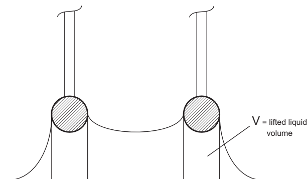
Fig. 2. Cross section of the ring with liquid lamella.
