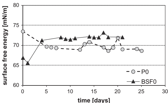
Fig. 5. Evolution of surface energy versus time (P0 and BFS0 mixes).
