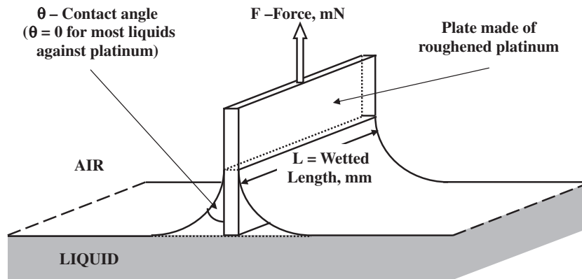
Fig. 3. Cross-section of the wetted plate.
