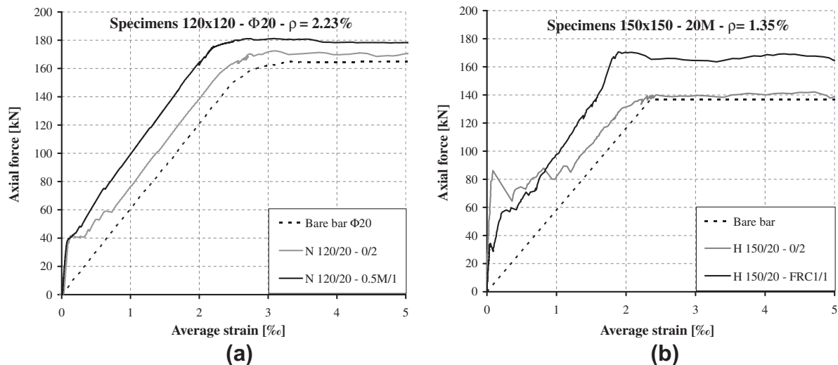
Fig. 3. Typical response of a NSRC and NSFRC (a) and HSRC and HSFR tie elements (b).
