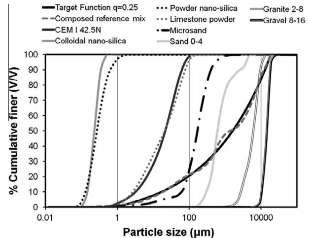
Fig. 1. PSD of the used materials, target function based on [36] and composition of reference mix (dashed line) for D_{min} = 60 nm.
