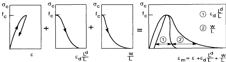
FIG. 2 Composition of the complete stress-strain curve
