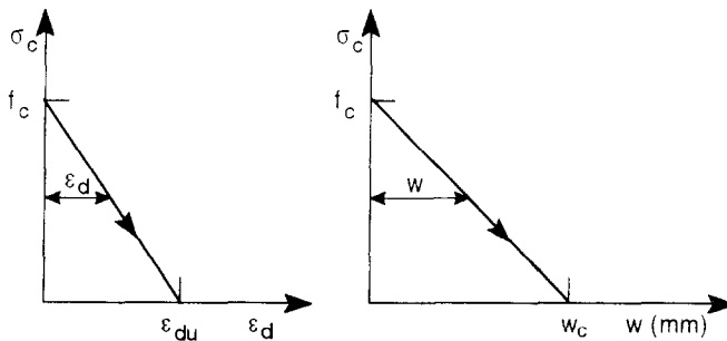
FIG. 3 Linear softening description
