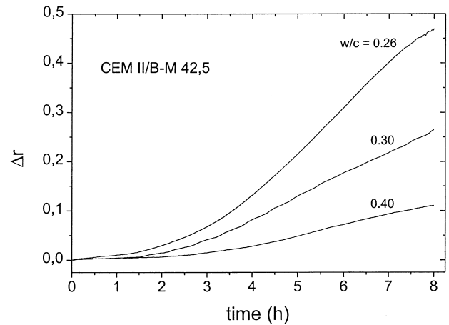
Fig. 3. The \Delta r change during the early hydration of CEM II/B-M 42,5 pastes with different w/c ratios.
