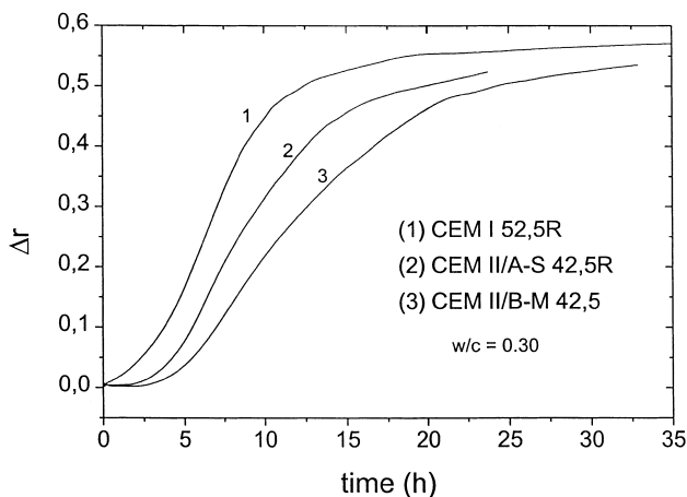
Fig. 2. The \Delta r change during the early hydration of three pastes made with different cements but with the same w/c ratio.
