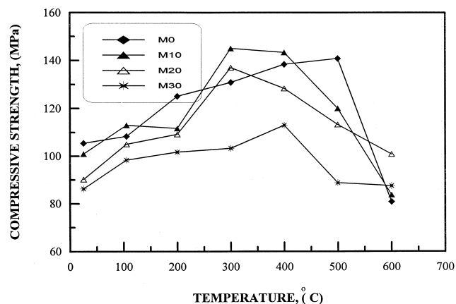
Fig. 2. Variations of compressive strength of cement pastes with temperature.
