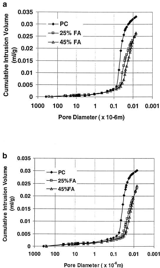
Fig. 3. Pore size distribution of the concrete mixes at w/b = 0.24: (a) 28 days and (b) 90 days.
