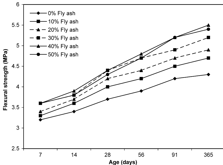
Fig. 5. Flexural strength versus age.
