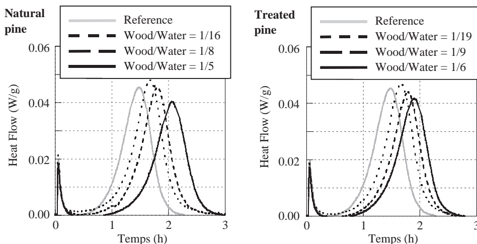
Fig. 1. The influence of the forest pine/water ratio on the hydration kinetics of plaster.
