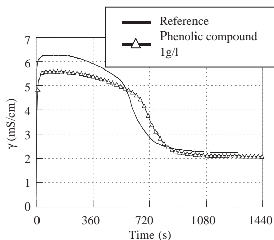
Fig. 8. The influence of aqueous solutions of phenolic substances.
