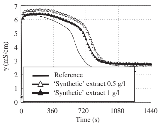
Fig. 9. The influence of aqueous solutions of a mixture of the most common molecules detected.
