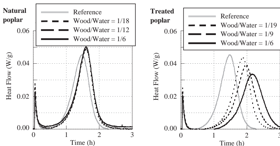
Fig. 2. The influence of the poplar/water ratio on the hydration kinetics of plaster.
