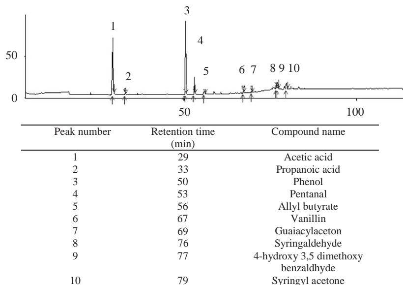
Fig. 5. Gaseous phase chromatogram of the treated poplar aqueous extracts.
