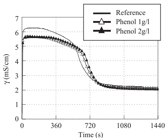
Fig. 7. The influence of aqueous solutions of phenol.
