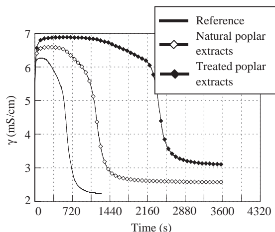
Fig. 3. The influence of the poplar extracts on the hydration kinetics of plaster—conductimetric analysis.
