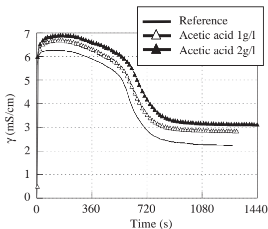
Fig. 6. The influence of acetic acid aqueous solutions on the hydration kinetics of plaster.
