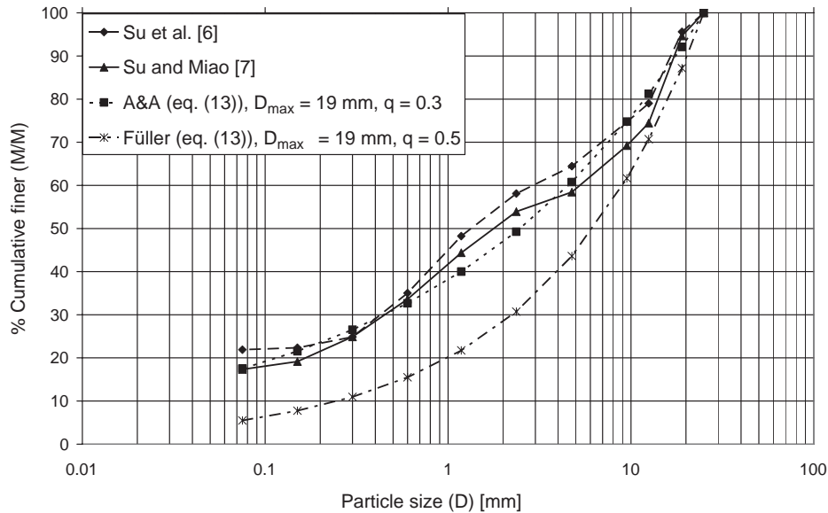
Fig. 6. Analysis of actual PSD of aggregates used by Su et al. [6] and Su and Miao [7].
