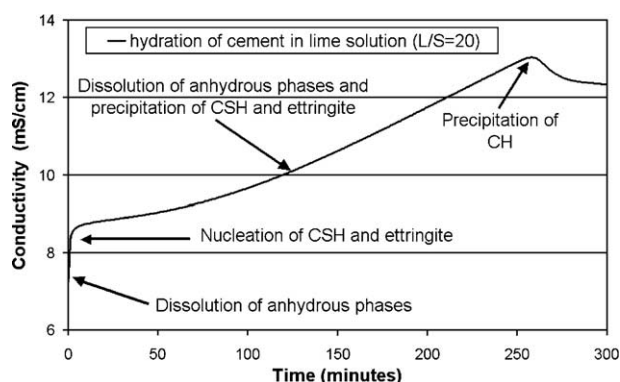
Fig. 2. Global view of hydration mechanism on a conductometric curve (ratio liquid to solid equal to 20).
