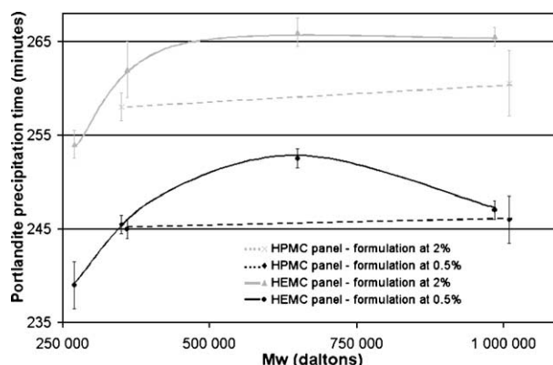
Fig. 6. Influence of M_w on portlandite precipitation delay in aqueous system.
