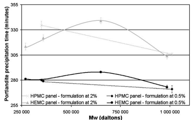
Fig. 10. Influence of M_w on portlandite precipitation delay in lime solution.
