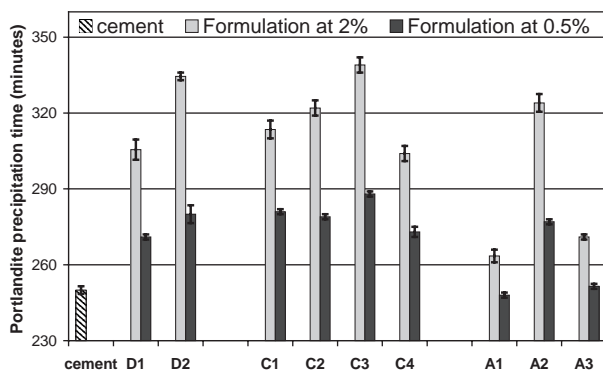
Fig. 8. Portlandite precipitation delay in lime solution (L/S=20).
