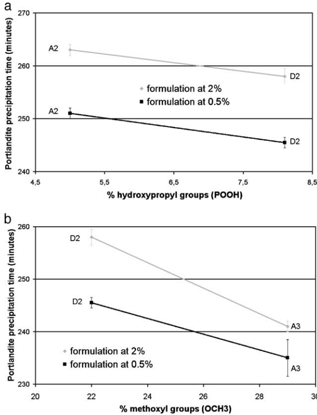
Fig. 7. Influence of % POOH (a) and % OCH 3 (b) on portlandite precipitation delay in aqueous system.
