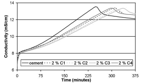
Fig. 9. Conductometric curves of cement admixed with 2% of C1 to C4 in lime solution.
