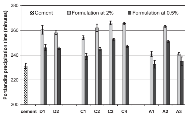
Fig. 4. Portlandite precipitation delay in aqueous system (L/S=20).
