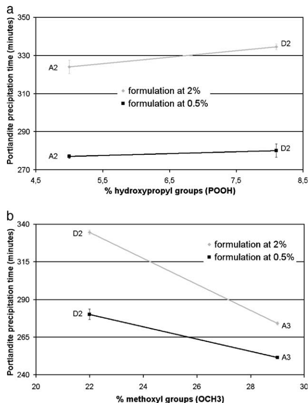
Fig. 11. Influence of % POOH (a) and % OCH 3 (b) on portlandite precipitation delay in lime solution.
