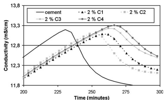
Fig. 5. Conductometric curves of cement admixed with 2% of C1 to C4 in aqueous system.
