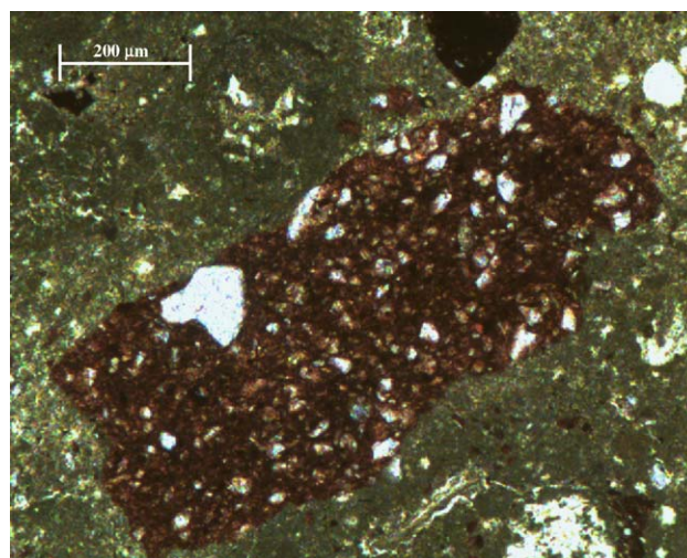
Fig. 1. Thin section photomicrograph (plane polars) of a historic lime mortar from the cathedral of Tournai (Belgium) with centrally in the image a ceramic fragment, without clear reaction rims.
