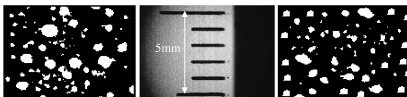
Fig. 7. Typical binary images (a) for cement–sand mix (b) scale (c) for cement–fly ash mix (100 % replacement level) (20X magnification).
