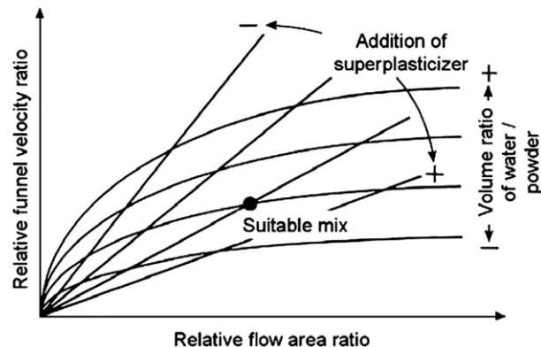
Fig. 35. Mix design by addition of superplasticizer and volume ratio of water/powder ratio [58].
