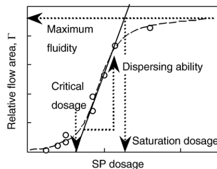
Fig. 21. Critical dosage and dispersing ability [22].
