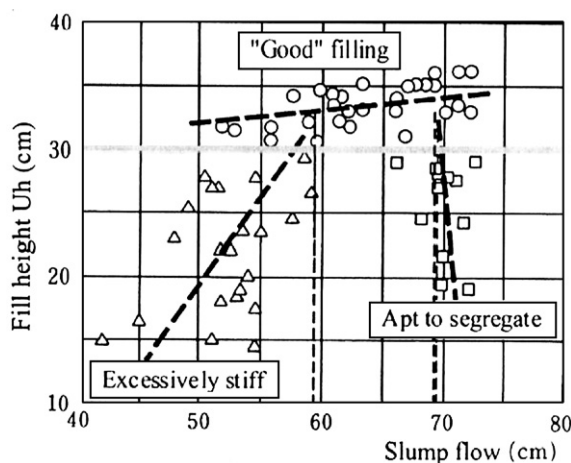
Fig. 37. Acceptable range of slump flow value of SCC with good self compacting concrete [61,62].
