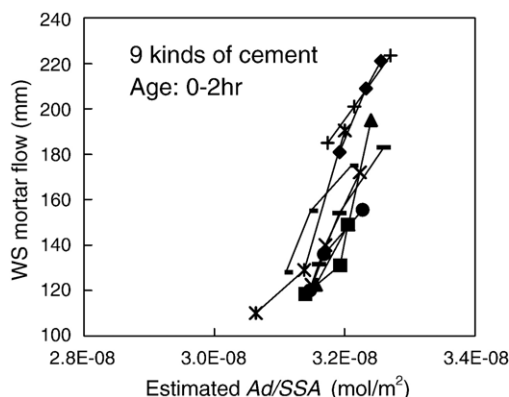
Fig. 14. Estimated \text{Ad/SSA} and \text{WS mortar flow} [23].
