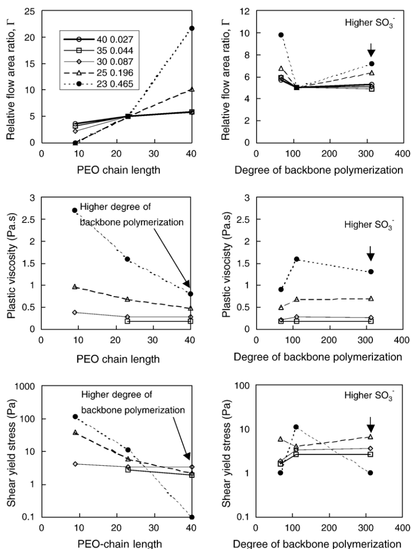
Fig. 9. The effects of chemical structure of PC on the rheological behavior of cement paste (Legend: W/C , dosage of PC) [22].
