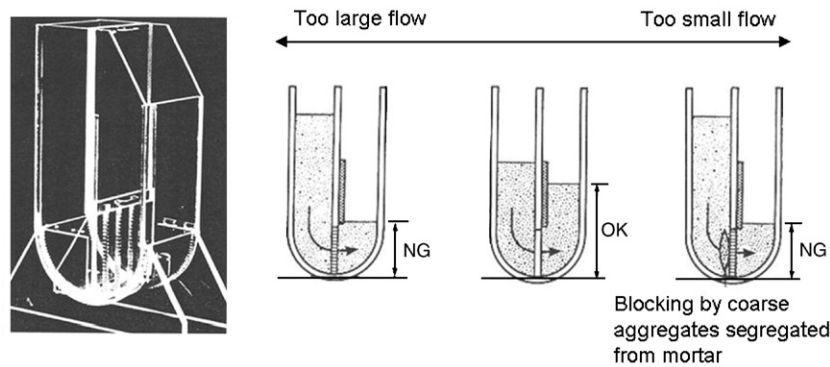
Fig. 36. U-shape test method apparatus (Shintosh method) [61,62].
