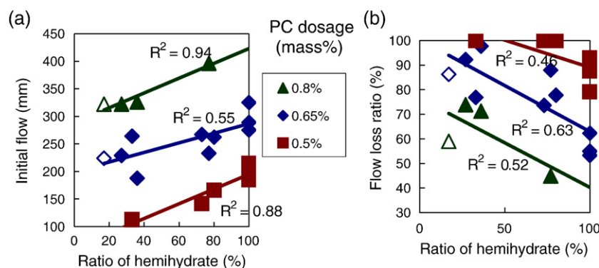
Fig. 28. Ratio of hemihydrate and initial flow (a) and flow loss ratio (b) [47].
