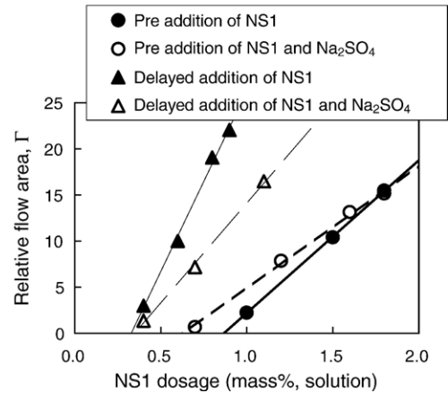
Fig. 26. The effect of delayed addition and alkali sulfate addition on the performance of PNS [45].
