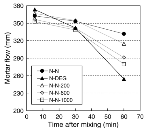
Fig. 32. The effect of DEG addition on the fluidity of mortar containing PC [49]. N-N: no grinding agent, N-DEG: 200 ppm of DEG addition during milling process, N-N-200, 600, 1000: 200, 600, and 1000 ppm of DEG addition to N-N after milling.
