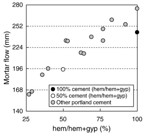
Fig. 29. The effect of hemihydrate ratio on the fluidity of mortar containing PC [46]. 100% and 50% is the ratio of hemihydrate in cement made in a plant. Other cement was made from one clinker in the laboratory.
