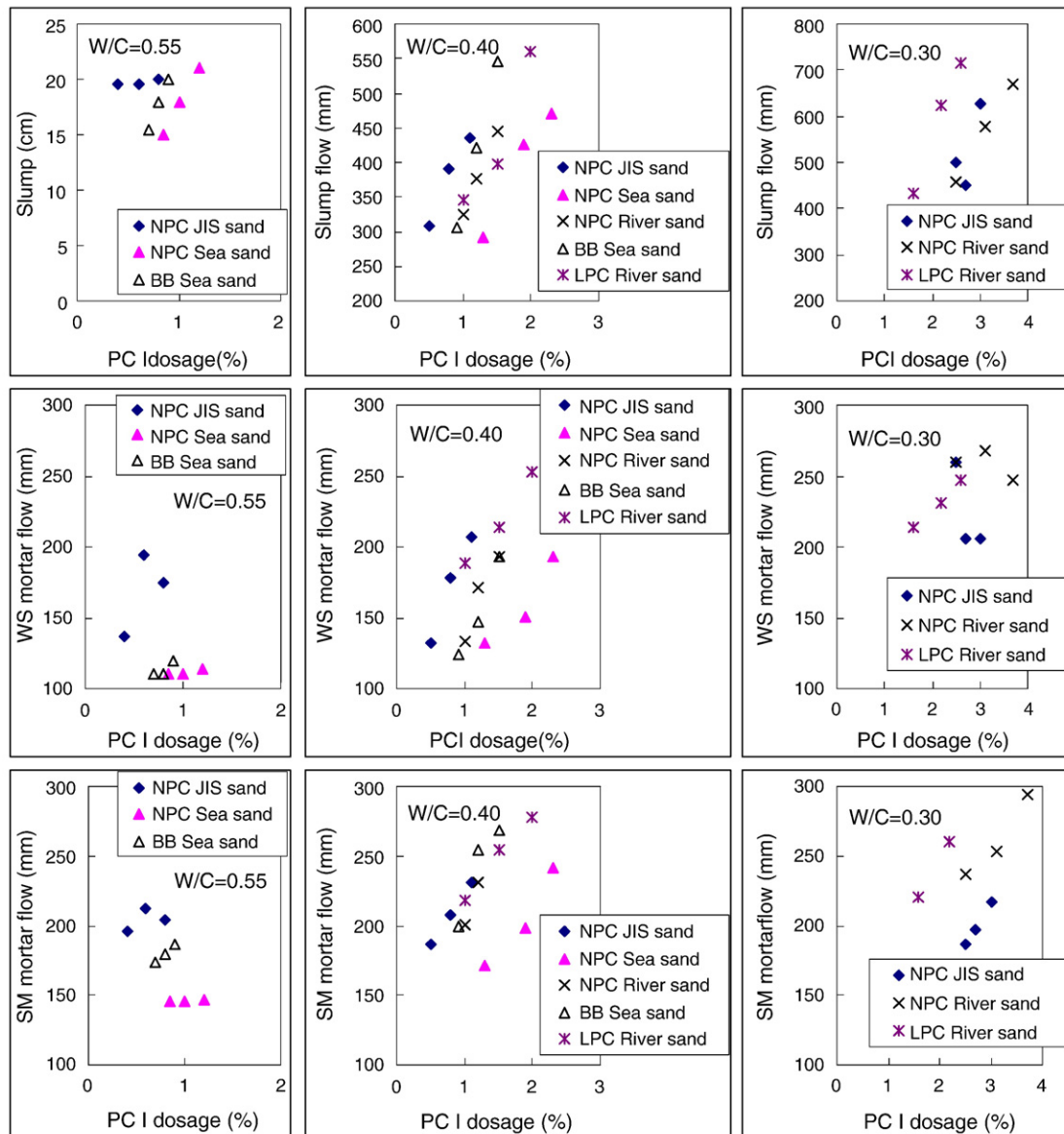
Fig. 17. Relationship between fluidity (concrete slump, wet screened mortar flow, and separately mixed mortar flow) and PC dosage at various W/C [39]. (NPC: Ordinary Portland cement, BB: 50% Blastfurnace slag cement, LPC: Low heat Portland cement).
