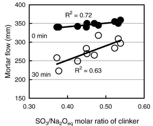
Fig. 31. Effect of SO_3/Na_2O_{eq} ratio of clinker on the fluidity of mortar containing PC [47].
