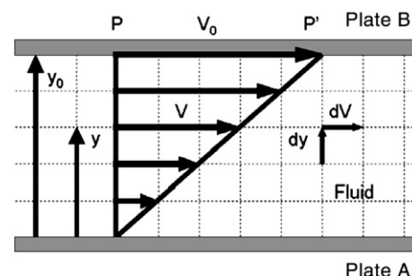
Fig. 1. Newtonian flow.
