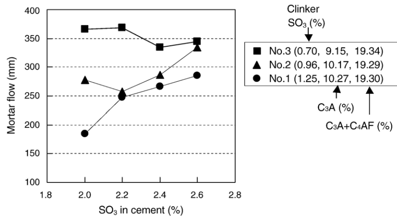
Fig. 27. Effect of SO 3 content in cement on the fluidity of mortar containing PC [46].
