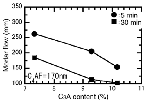
Fig. 30. C_3A content and the fluidity of mortar containing PC [48].
