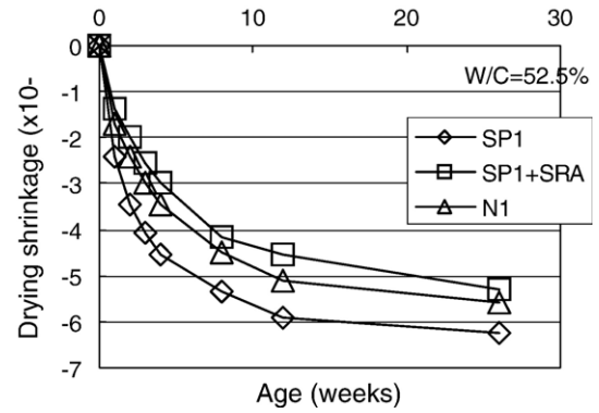
Fig. 8. Drying shrinkage reduction by multi-function-type superplasticizer [20].
