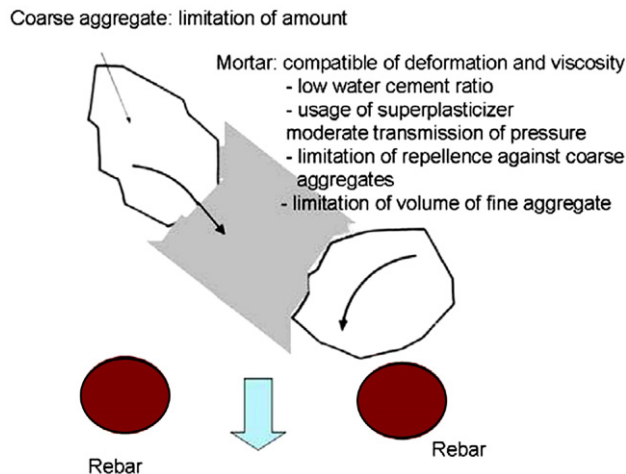
Fig. 33. An image on the self-compactibility of fresh concrete, focusing on the mechanism of passing through the gap [58].
