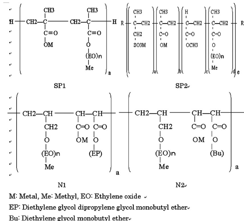
Fig. 7. Chemical structure of multi-function-type superplasticizer [20].
