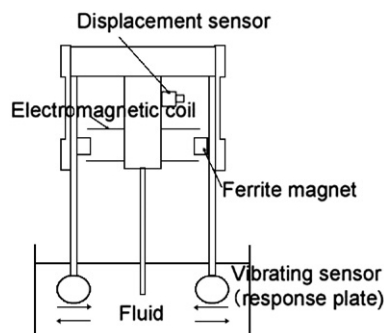
Fig. 3. Schematic diagram of vibrating viscometer.
