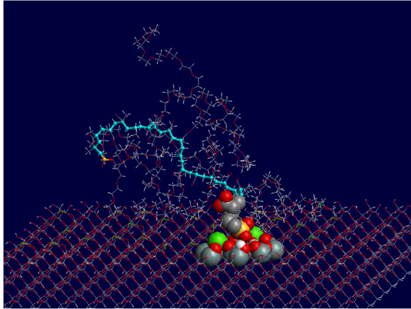
Fig. 10. Steric conformation of adsorbed PC at Ca site on model hydrate [23].
