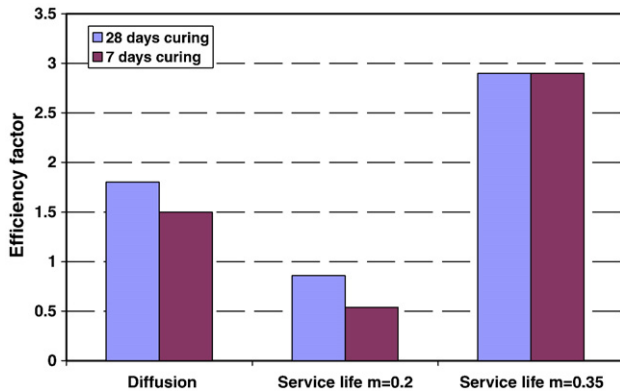
Fig. 14. Fly ash efficiency k -factors for durability of steel corrosion in concrete in chloride environment, after Bentur [12].
