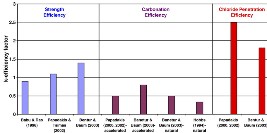
Fig. 6. k -efficiency factors for strength, carbonation and chloride penetration for 90 days of fly ash concretes, based on data compiled from the literature, after Bentur [12].
