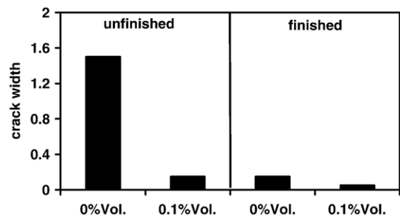
Fig. 4. Effect of fibrillated polypropylene fibre and mode of finishing on plastic shrinkage cracking, after Soroushian et al. [5].
