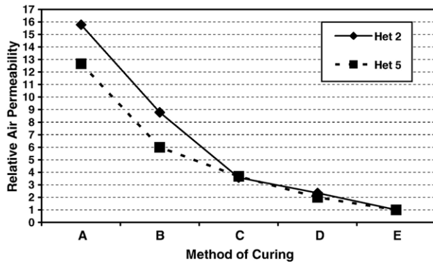
Fig. 5. Effect of curing method on the relative air permeability coefficient of the concrete cover in a simulated laboratory test, for 20 MPa (Het 2) and 50 MPa (Het 5) concretes, after Kubens et al. [8]. E — 28 days water ponding curing; D — 7 days ponding water curing; C — 7 days of intermittent water curing; B — 3 days of intermittent water curing, A — continuous air curing after demolding at 1 day.
