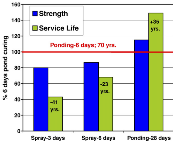
Fig. 2. The effect of curing conditions on strength and service life in carbonating conditions, relative to curing by ponding for 6 days. The concrete strength is 50 MPa (100 mm air dry cubes), after Bentur [3].
