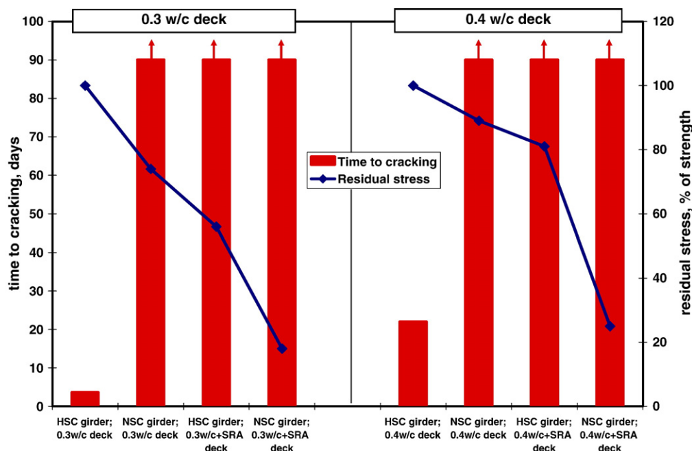
Fig. 11. Time to cracking and residual stresses in bridge decks, compiled from the data in Li et al. [48,49] for 0.3 and 0.4 w/c ratio deck concrete, with and without shrinkage reducing admixture (SRA), cast on girders which are made from prestressed normal or high strength concretes (NSC and HSC, respectively). Modeling runs were carried out up to 90 days, and thus the 90 days bars indicate that no cracking occurred within that time period.
