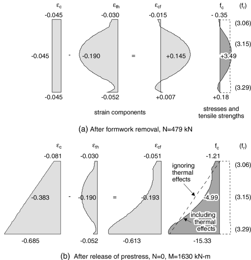
Fig. 13. Predicted concrete strains and stresses in precast pretensioned girder.
