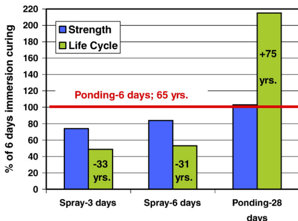
Fig. 3. The effect of curing conditions on strength and service life in chloride conditions, relative to curing by ponding for 6 days. The concrete strength is 75 MPa (100 mm air dry cubes), after Bentur [3].
