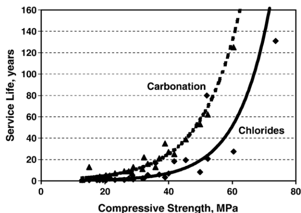
Fig. 1. Calculated service life of a reinforced concrete structure for carbonation and chloride steel induced corrosion, after Bentur [3].
