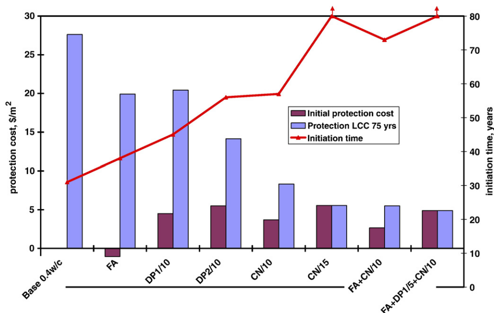
Fig. 15. Prediction of costs (initial and life cycle) and corrosion initiation times for a bridge deck with 75-year design life, after Bentur et al. [59].
