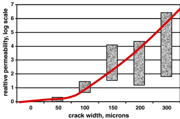
Fig. 9. Effect of crack width on the relative permeability of water flow, based on compilation from the literature (Aldea et al. [39,40], Evardsen [41], Reinhardt and Jooss [43], Schiessl and Raupach [44], Burlion et al. [42]).
