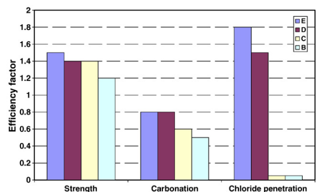
Fig. 7. Effect of curing on the 90 days efficiency factor of type F fly ash determined for strength, carbonation and chloride penetration; E — 28 days water ponding curing; D — 7 days ponding water curing; C — 7 days of intermittent water curing; B — 3 days of intermittent water curing, based on the data in Bentur and Baum [4].
