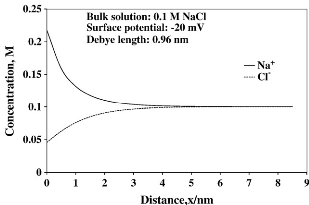
Fig. 5. Ionic distribution near a charged surface. The surface is in contact with 0.1 M NaCl.
