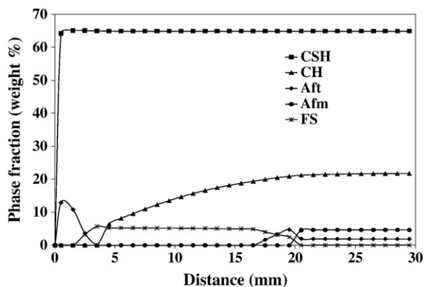
Fig. 13. Simulated main cement hydrate distribution in HCP after 91 days of seawater exposure.
