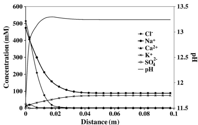
Fig. 6. Simulated ionic concentration in the free solution of pores (centre of pore) considering ionic adsorption.
