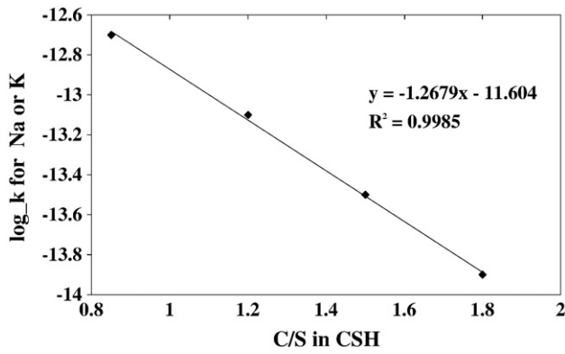
Fig. 4. Change of \log_k with C/S ratio of C–S–H for adsorption of sodium or potassium.
