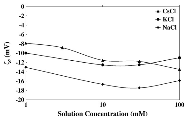
Fig. 2. Measured \zeta of HCP suspensions in chloride solutions.
