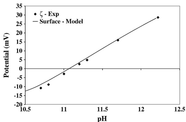
Fig. 1. Measured \zeta and calculated surface potential of C-S-H as a function of pH in calcium hydroxide solution.
