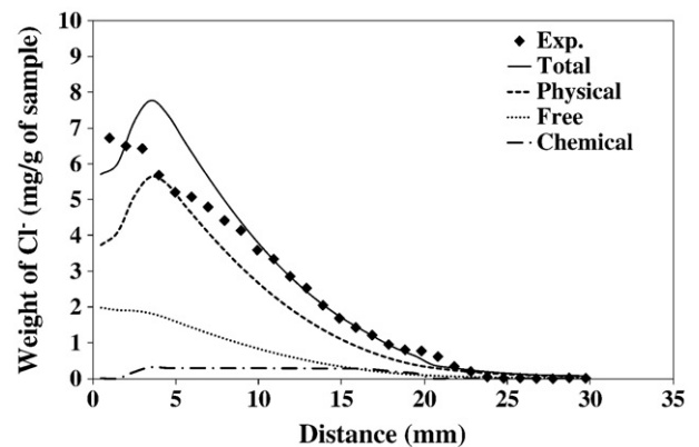
Fig. 12. Comparison between experimental and simulated chloride profiles for HCP after 91 days of seawater exposure.
