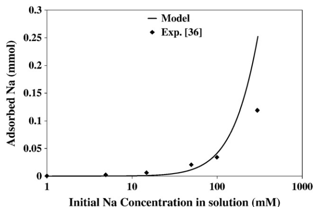
Fig. 3. Measured [36] and predicted adsorption of sodium on C-S-H for C/S ratio of 1.5 as function of sodium concentration.
