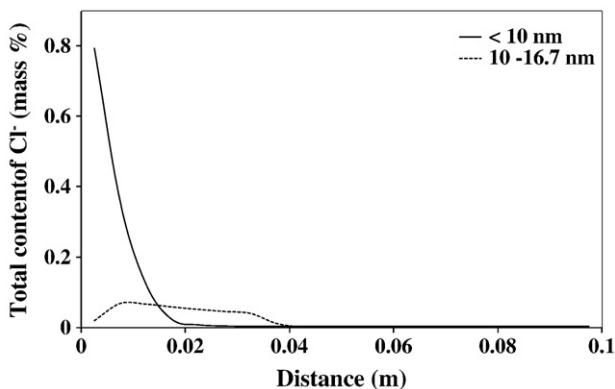
Fig. 10. Simulated results for dependence of pore size on total content of chloride.
