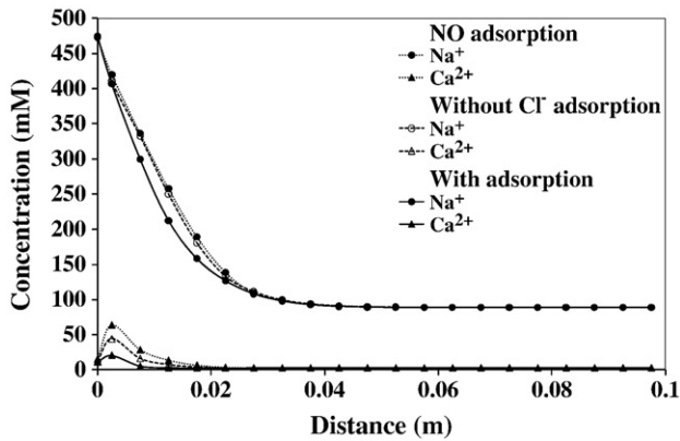
Fig. 9. Simulated results for dependence of physical adsorption on cation transport.
