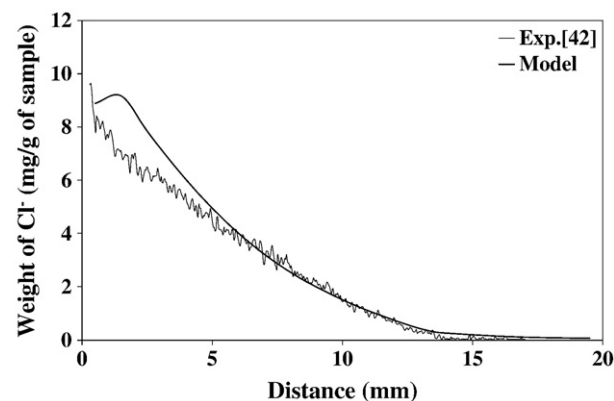
Fig. 15. Comparison between experimental [42] and simulated chloride profiles for HCP after 30 days of chloride exposure.
