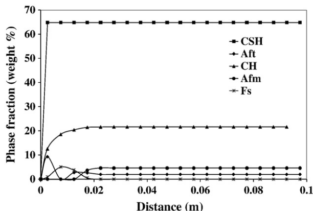
Fig. 7. Main cement hydrate distribution during multi-ionic transport in HCP.
