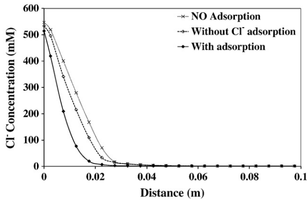
Fig. 8. Simulated results for dependence of physical adsorption on chloride transport.
