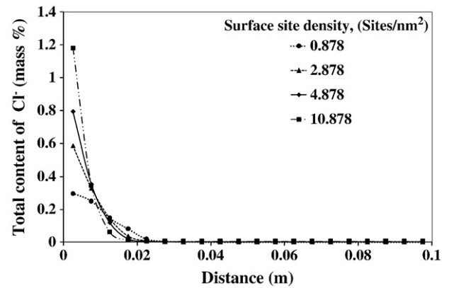
Fig. 11. Simulated results for dependence of surface site density on total content of chloride.
