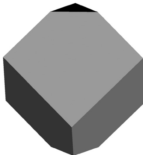
Fig. 9. Calculated equilibrium morphology of portlandite in water. Dark gray: [00.1] facet, light gray: [20.3] facet.
