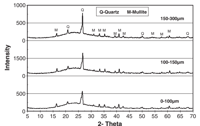
Fig. 2. X-ray diffraction spectra of the cenosphere material of different size fractions.
