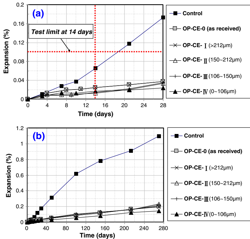
Fig. 6. Expansion of the mortar bars determined according to ASTM C1260 test: (a) up to 28 days; (b) up to 9 months.
