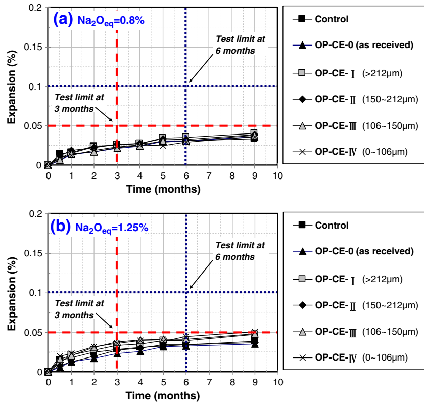
Fig. 5. Expansion of the mortar bars determined according to ASTM C227 test: (a) Na 2 O eq = 0.8%; (b) Na 2 O eq = 1.25%.
