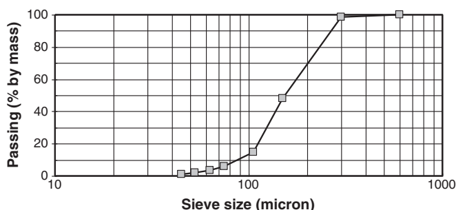
Fig. 1. Particle size distribution of the cenospheres.
