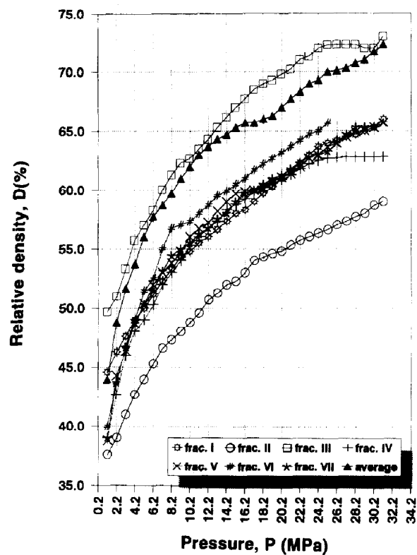
Fig. 1. Compaction response diagrams of fractions I–VII and the average sample.
