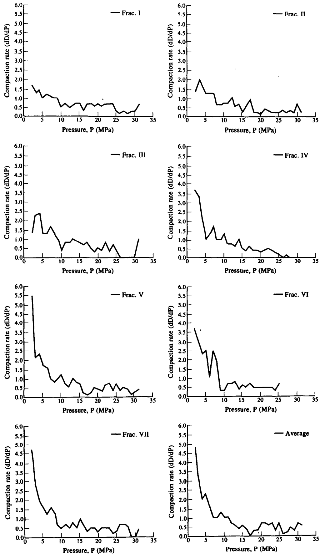
Fig. 2. Compaction rate diagrams of fractions I-VII and the average sample.
