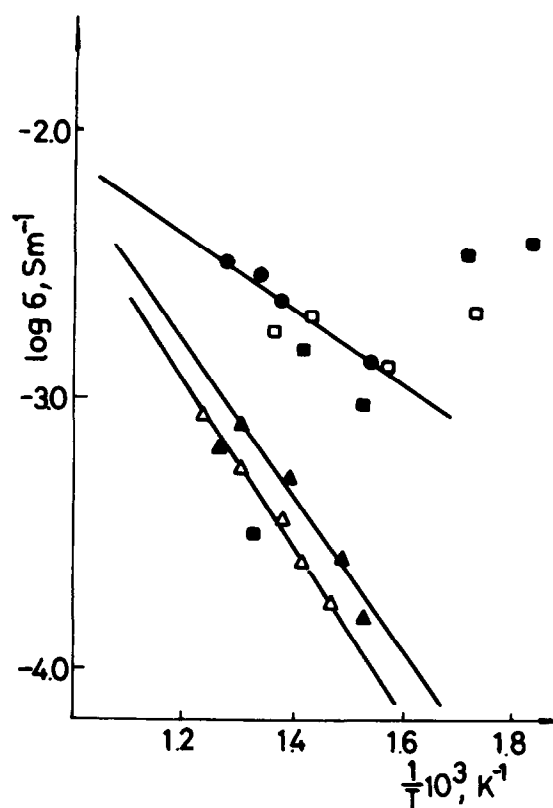
Fig. 2. Conductivity measurements in the form of an Arrhenius plot for zeolite \text{Ag}_x\text{Na}_{85-x}\text{-X} . D samples: x = 9.4 (●), x = 20.1 (△), x = 55.6 (▲), ND samples: x = 9.4 (■), x = 20.1 (□).
