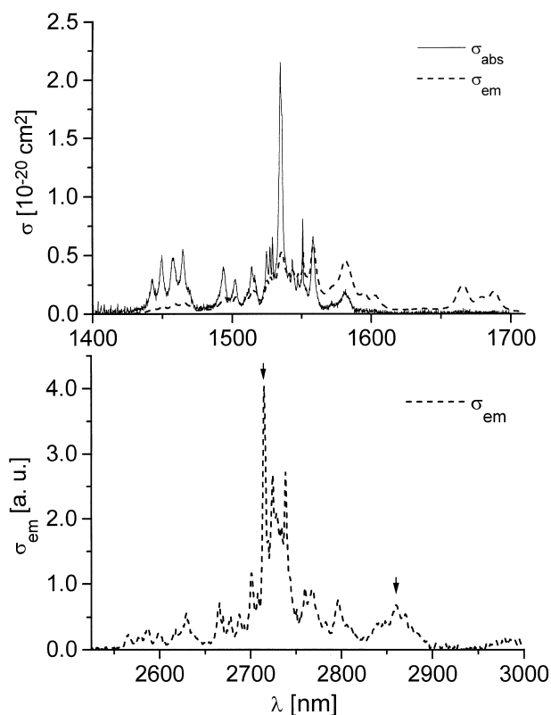
Fig. 2. Absorption and emission cross-sections of Er:Sc 2 O 3 . The arrows indicate the laser lines near 3 \mu m.
