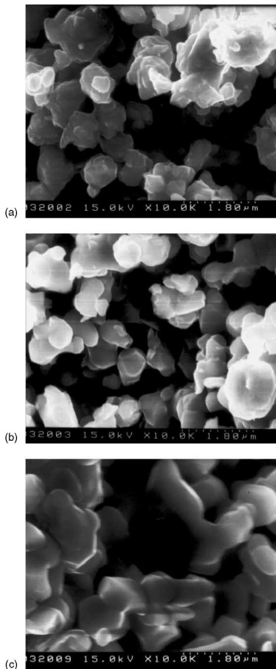
Fig. 7. SEM micrographs of \text{ZnTiO}_3 powders calcined at 800 °C for (a) 24 h, (b) 48 h, and (c) 72 h in air.
