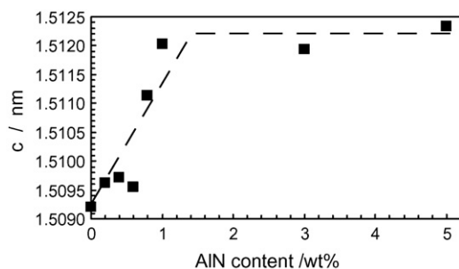
Fig. 2. Change in lattice parameter in SiC ceramics against aluminum nitride adding amount.
