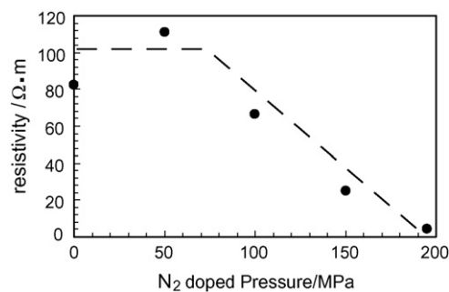
Fig. 4. Change in resistivity without load in 1 and 3 wt.% aluminum nitride doped SiC ceramics against nitrogen doping pressure.
