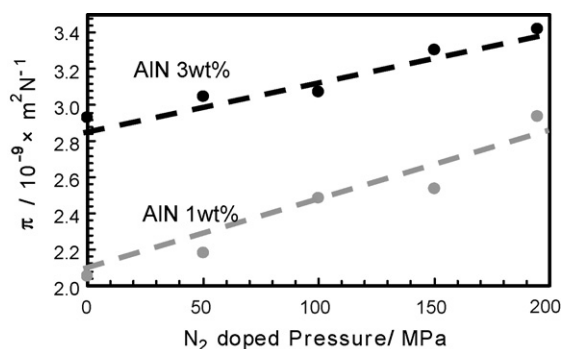
Fig. 5. Change in piezoresistive coefficient in 1 and 3 wt.% aluminum nitride doped SiC ceramics against nitrogen doping pressure.
