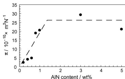
Fig. 3. Change in piezoresistive coefficient in SiC ceramics against aluminum nitride adding amount.
