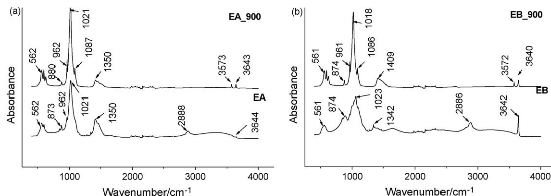
Fig. 3. FTIR spectra of the samples: (a) EA and EA_900, (b) EB and EB_900.
