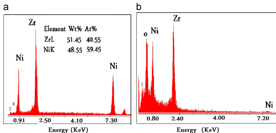
Fig. 5. EDS spectra of \text{Ni}_{60}\text{Zr}_{40} alloy: (a) alloy quenched in liquid nitrogen and (b) the same alloy after oxidation at 1073 K under oxygen atmosphere for 2 h.
