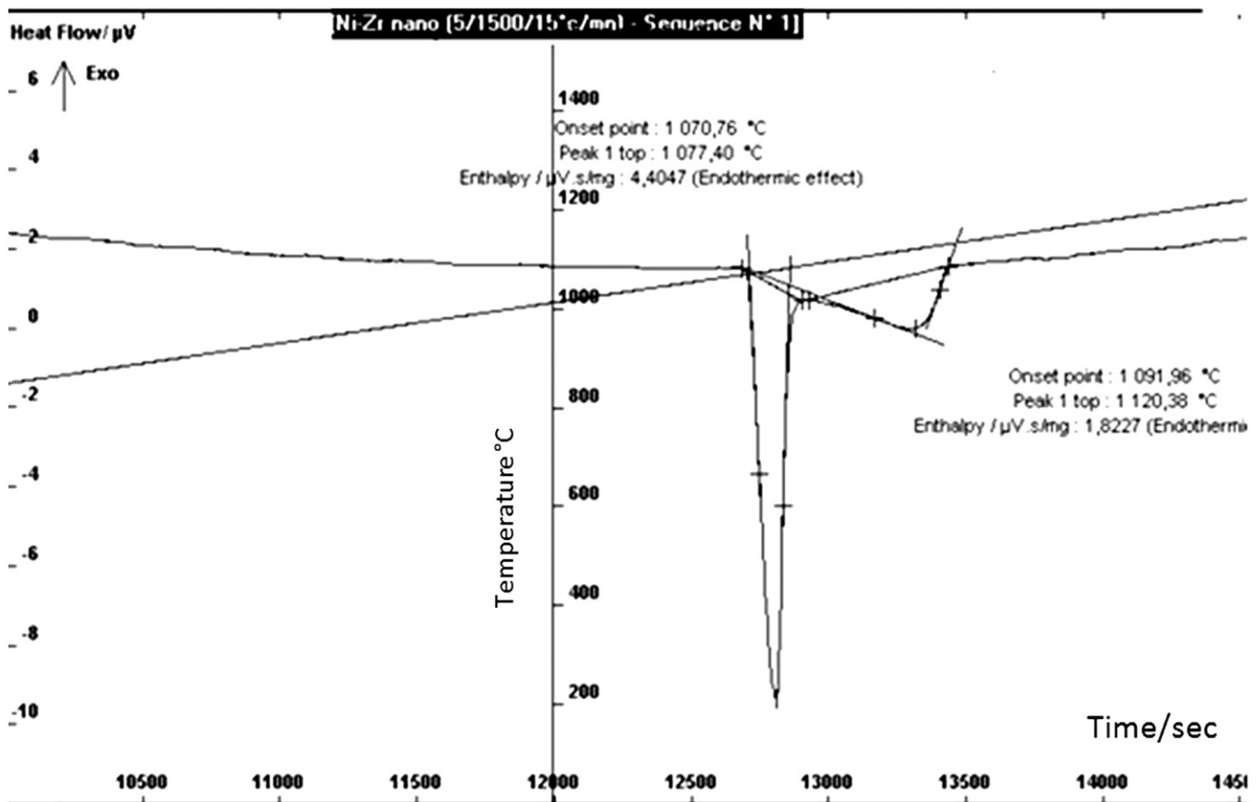
Fig. 4. DTA curves of \text{Ni}_{60}\text{Zr}_{40} quenched alloy with a heating rate of 5 K/min. Two endothermic peaks, characterizing the amorphous state of the quenched material, emerge (at the top peaks located at 1350 and 1393 K).
