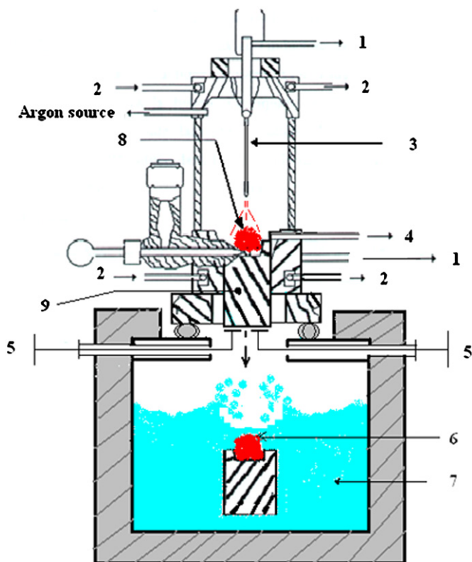
Fig. 1. Experimental set-up illustrating alloy preparation and quenching in liquid nitrogen: 1, generator (+, –); 2, into the cooler; 3, electrode (W); 4, vacuum frame; 5, trap; 6, sample quenched in liquid nitrogen; 7, liquid nitrogen vat; 8, sample in fusion; 9, crucible.
