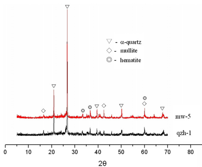
Fig. 3. XRD diagram of typical Zisha samples.
