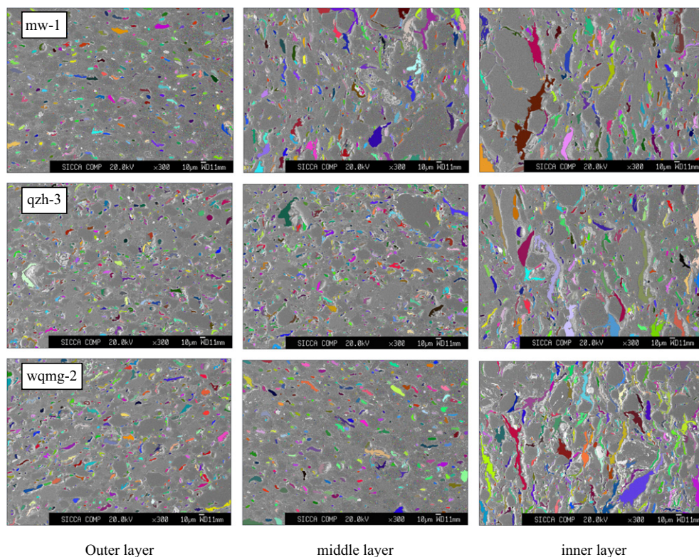
Fig. 4. The distribution of pores in different layers of typical Zisha samples (Note: the porosity of the outer layer is 5–9%, that of the middle layer is 9–14% and that of the inner layer is 15–17%).
