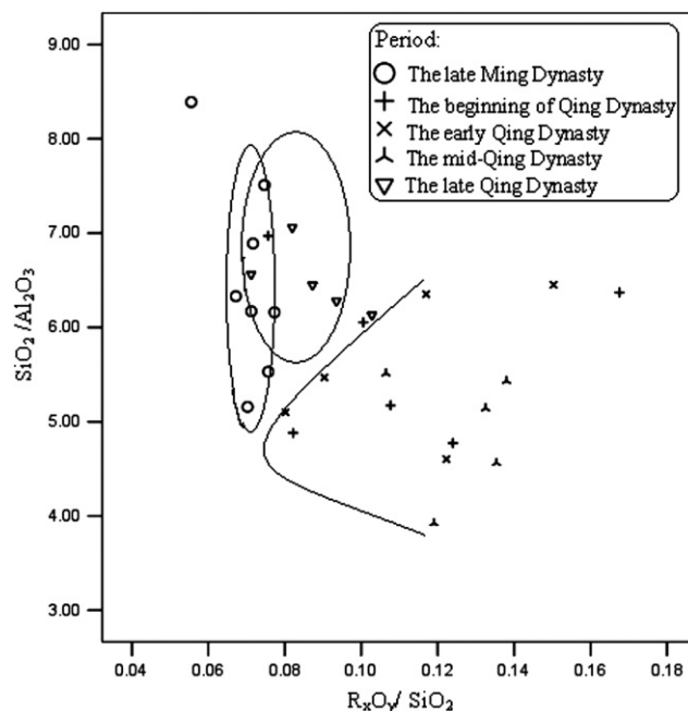
Fig. 5. Scatter diagram of the \text{SiO}_2/\text{Al}_2\text{O}_3 and R_x\text{O}_y/\text{SiO}_2 of Zisha samples.
