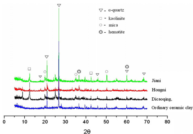
Fig. 2. XRD diagram of Zisha raw material and ordinary ceramic clay.
