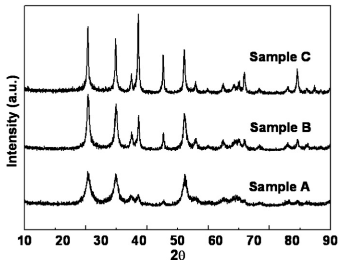
Fig. 2. XRD plots obtained from samples A, B, and C after calcination.
