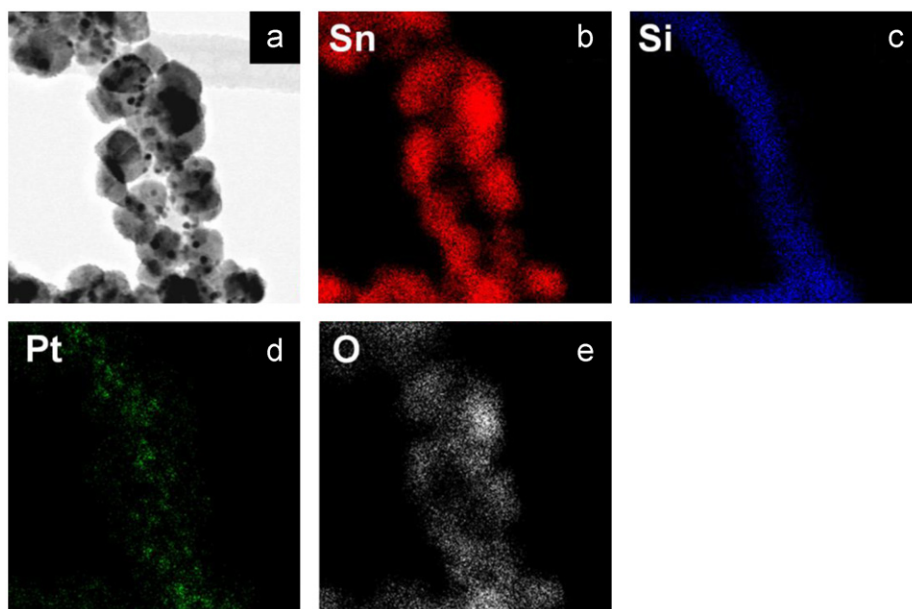
Fig. 5. TEM-EDS mapping data obtained from sample A.
