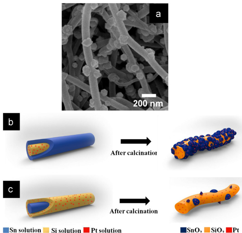
Fig. 7. SEM image of non-uniform composite NFs obtained from an experimental method of Fig. 1(b). (a). Schematic of uniform composite NFs (b) and non-uniform composite NFs (c) depending on the position of the precursor solutions in co-electrospinning.
