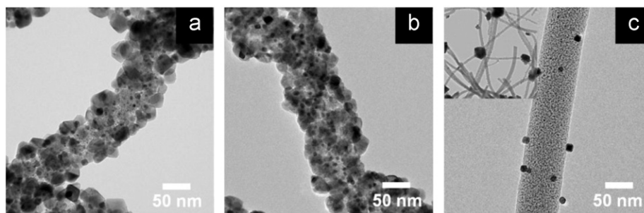
Fig. 4. TEM images of samples A, B, and C after calcination ((a)–(c)).
