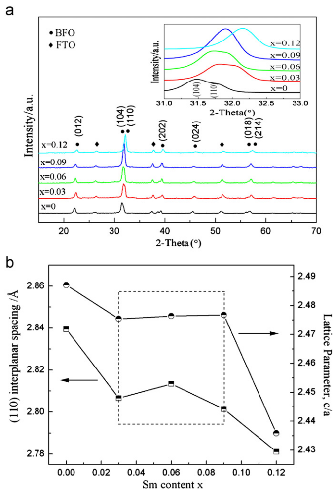
Fig. 1. XRD patterns of \text{Bi}_{1-x}\text{Sm}_x\text{FeO}_3 films at room temperature. (a) XRD patterns of \text{Bi}_{1-x}\text{Sm}_x\text{FeO}_3 films at the range of 31°–33°; (b) unit cell parameter of \text{Bi}_{1-x}\text{Sm}_x\text{FeO}_3 thin films as a function of Sm doping content.
