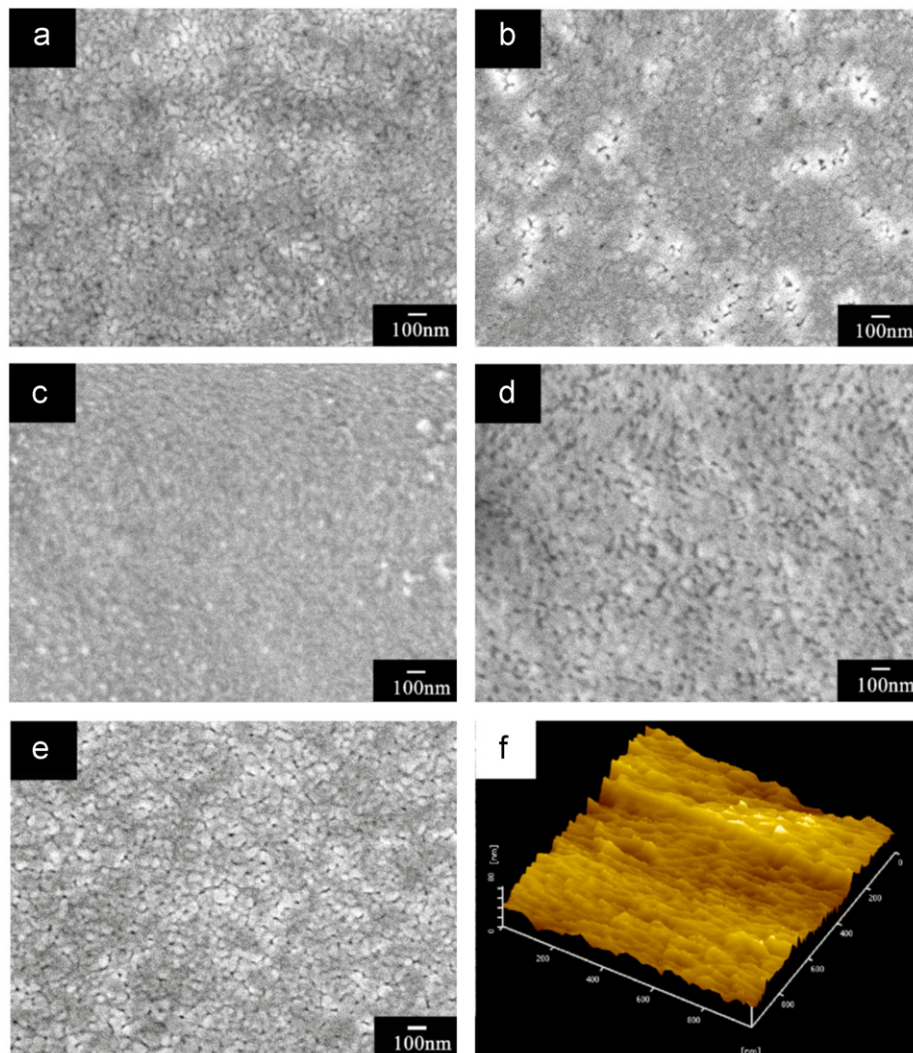
Fig. 2. FE-SEM images and AFM image of Bi 1-x Sm x FeO 3 films (a) x=0 , (b) x=0.03 , (c) x=0.06 , (d) x=0.09 , (e) x=0.12 , and (f) x=0.09 .
