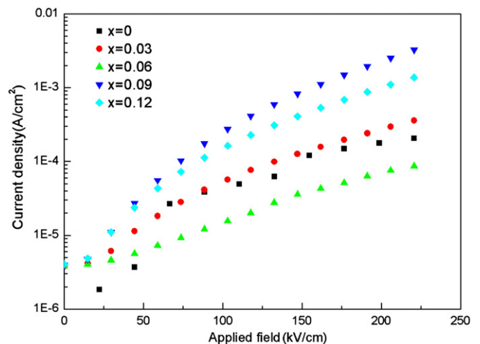
Fig. 4. Leakage current density of \text{Bi}_{1-x}\text{Sm}_x\text{FeO}_3 films as a function of applied voltage at room temperature.
