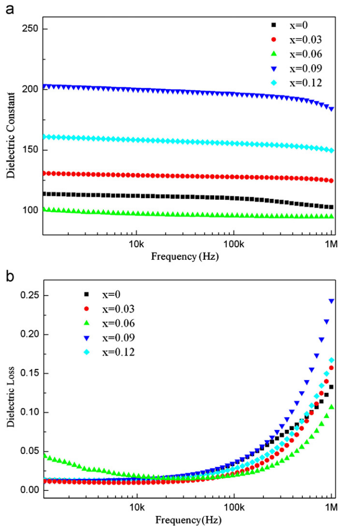
Fig. 3. (a) Dielectric constant and (b) dielectric loss of \text{Bi}_{1-x}\text{Sm}_x\text{FeO}_3 films as a function of frequency at room temperature.
