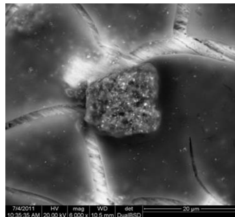
Fig. 1. SEM micrograph of the 22ZN powder before attrition milling. \text{Al}_2\text{O}_3 (the darker phase) and \text{ZrO}_2 (the brighter phase).
