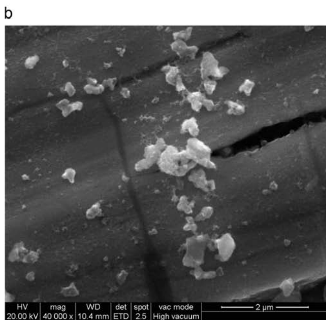
Fig. 4. SEM micrographs of different powders: (a) 10.5 ZN and (b) 22ZN.
