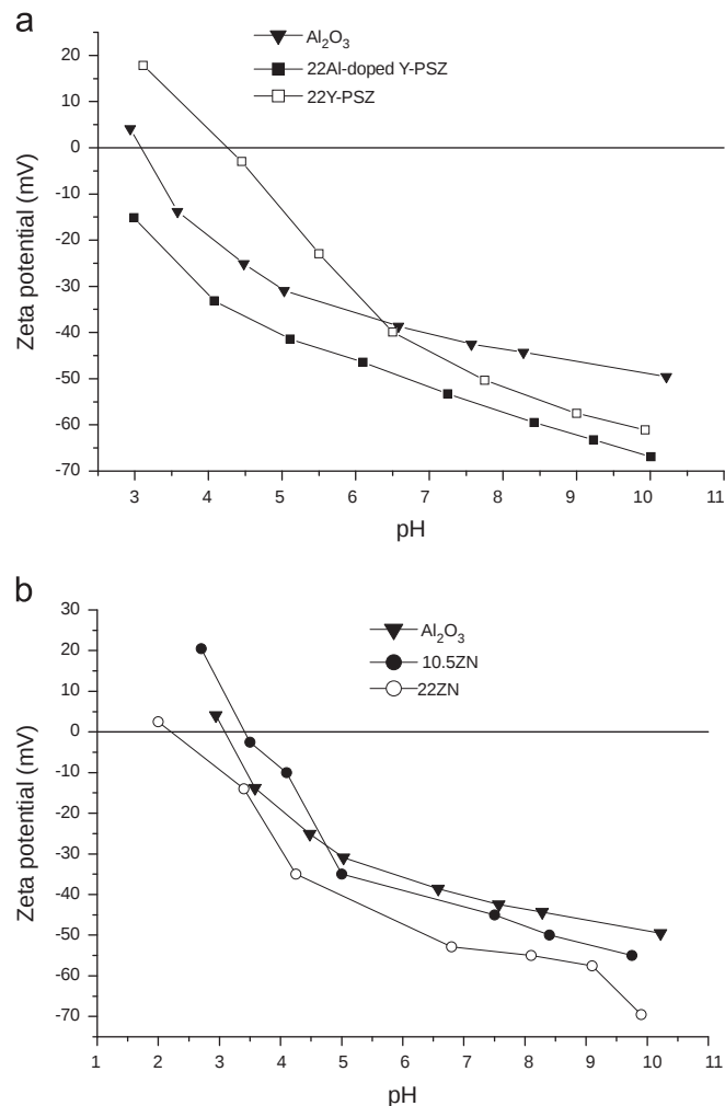
Fig. 8. Zeta potential vs. pH curves of different powders dispersed in slips with the optimum amount of \text{NH}_4\text{PA} solution added: (a) \text{Al}_2\text{O}_3 , 22Al-doped Y-PSZ and 22Y-PSZ, and (b) \text{Al}_2\text{O}_3 , 10.5ZN and 22ZN.
