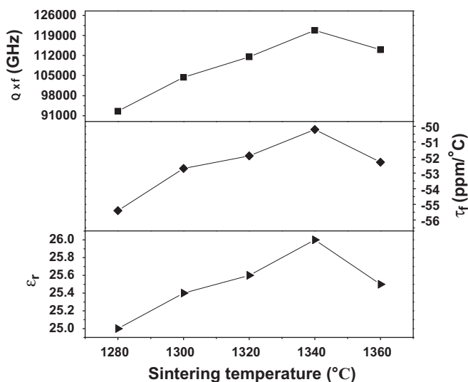
Fig. 4. The variation of the \epsilon_r , Q \times f and \tau_f values of \text{MgZrNb}_2\text{O}_8 ceramics sintered at different temperatures.
