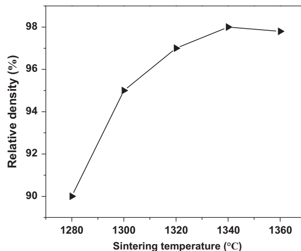
Fig. 2. The variation of the relative density of \text{MgZrNb}_2\text{O}_8 ceramics sintered at different temperatures.
