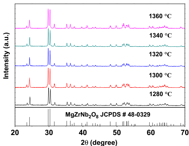
Fig. 1. The XRD patterns of \text{MgZrNb}_2\text{O}_8 ceramics sintered at different temperatures, as compared to the standard pattern of \text{MgZrNb}_2\text{O}_8 .
