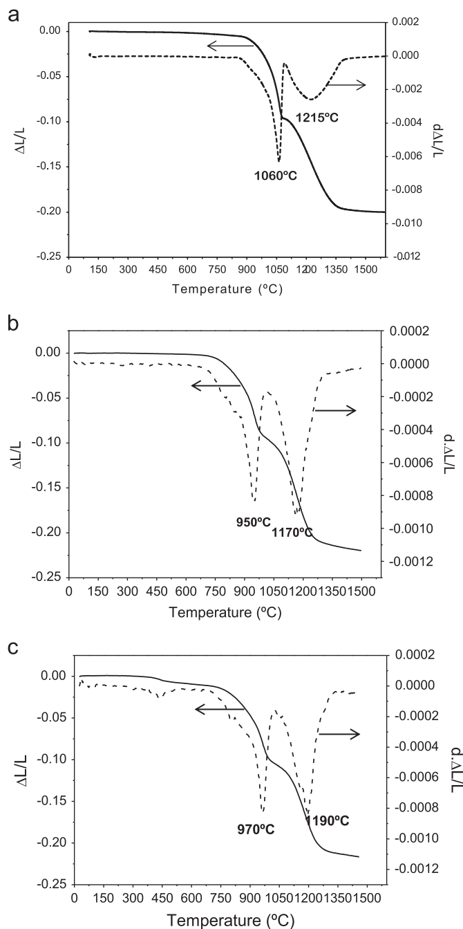
Fig. 6. Dilatometry curves and derivatives of 30M (a), bimodal 15P15M (b), and 3-components 10W5P15M (c) specimens.
