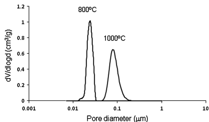
Fig. 9. Pore diameter distribution of 10W5P15M samples quenched at 800 °C and 1000 °C.
