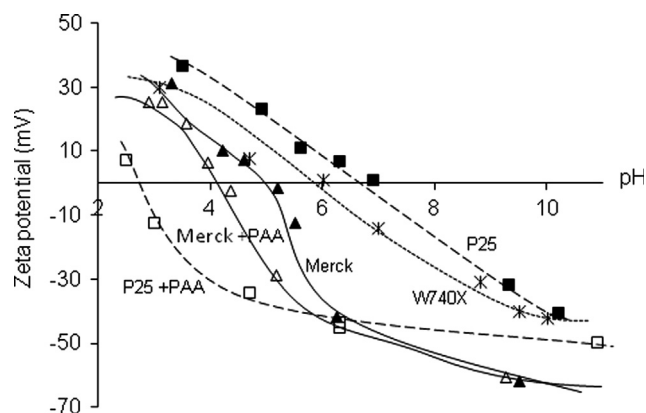
Fig. 2. Variation of zeta potential with pH of the starting powders as received and after the addition of the optimum deflocculant content.
