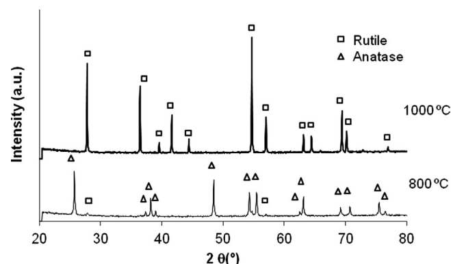
Fig. 7. XRD patterns of 10W5P15M samples quenched at 800 °C and 1000 °C.
