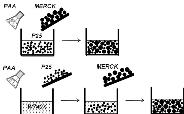
Fig. 1. Scheme of the procedure followed to prepare the suspensions of the mixtures.
