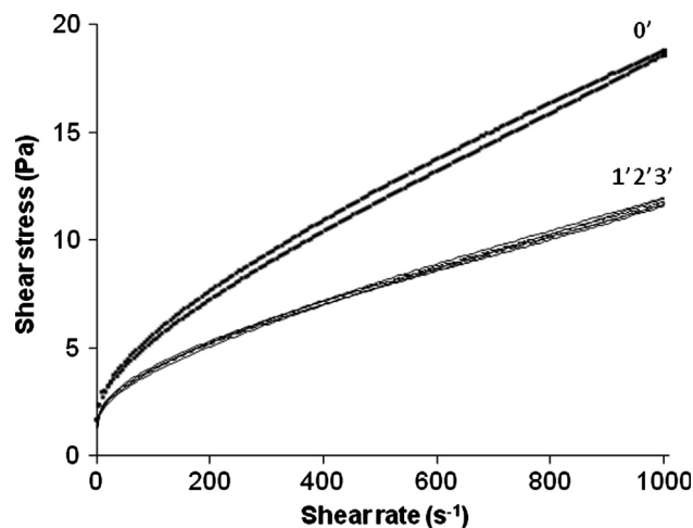
Fig. 3. Flow curves of 30M suspensions prepared with different US times.
