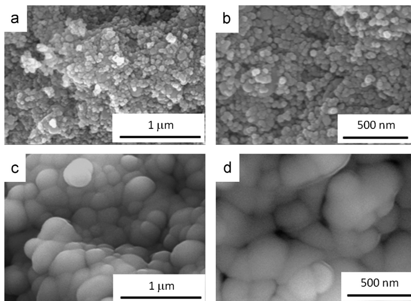
Fig. 8. FE-SEM microphotographs of 10W5P15M samples quenched at 800 °C (a and b) and 1000 °C (c and d).
