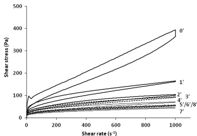
Fig. 4. Flow curves of bimodal 15P15M suspensions prepared with different US times.
