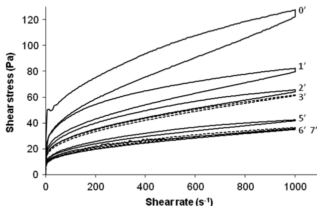
Fig. 5. Flow curves of 3-components 10W5P15M suspensions prepared with different US times.
