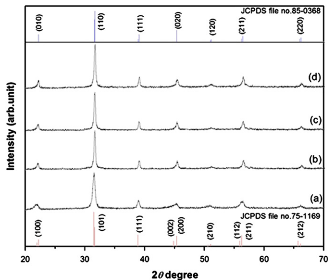
Fig. 1. XRD patterns of (La, K)-doped 0.75BiFeO 3 –0.25BaTiO 3 ceramics with fixed La of 1 mol% and varied K of (a) 0.5, (b) 1.0, (c) 3.0 and (d) 5.0 mol% K content. (For interpretation of the references to color in this figure legend, the reader is referred to the web version of this article.)
