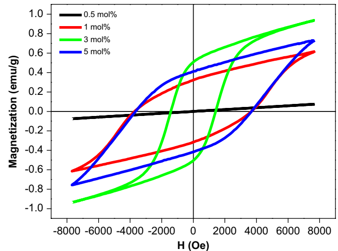
Fig. 4. M – H loops of (La, K)-doped 0.75\text{BiFeO}_3\text{--}0.25\text{BaTiO}_3 ceramics with fixed La of 1 mol% and varied K of 0.5, 1.0, 3.0 and 5.0 mol%. (For interpretation of the references to color in this figure legend, the reader is referred to the web version of this article.)
