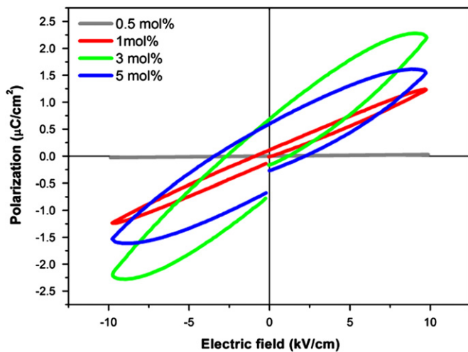
Fig. 3. P – E loops of (La, K)-doped 0.75\text{BiFeO}_3\text{--}0.25\text{BaTiO}_3 ceramics with fixed La of 1 mol% and varied K of 0.5, 1.0, 3.0 and 5.0 mol%. (For interpretation of the references to color in this figure legend, the reader is referred to the web version of this article.)
