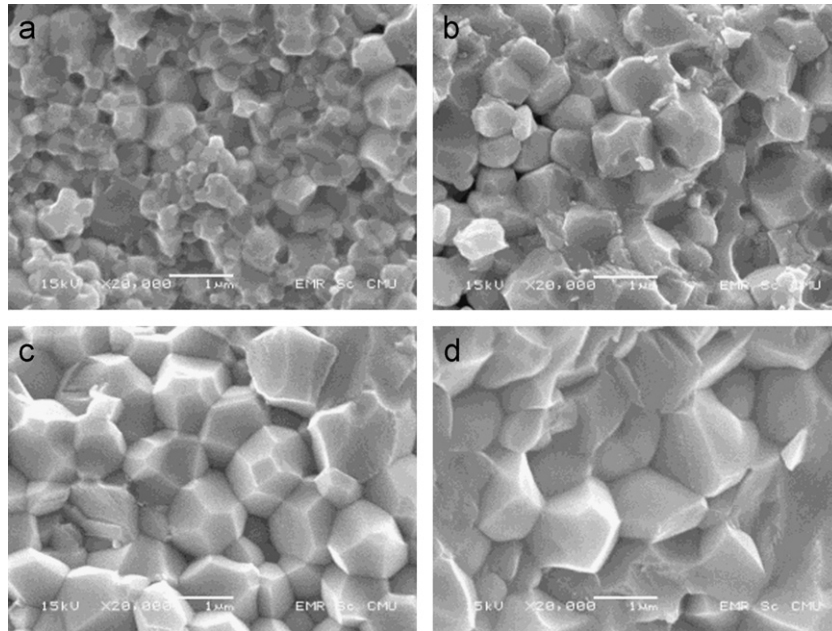
Fig. 2. SEM micrographs of (La, K)-doped 0.75\text{BiFeO}_3\text{--}0.25\text{BaTiO}_3 ceramics, with fixed La of 1 mol% and varied K of (a) 0.5, (b) 1.0, (c) 3.0 and (d) 5.0 mol%. (For interpretation of the references to color in this figure legend, the reader is referred to the web version of this article.)
