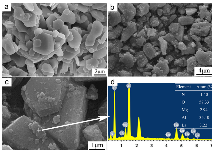
Fig. 4. FESEM micrographs and EDS patterns of as-prepared LaMgAl_{11}O_{19} and nitrided LaMgAl_{11}O_{19} phosphors. (a) SEM image of LaMgAl_{11}O_{19} , (b) SEM image of nitrided LaMgAl_{11}O_{19} , (c) surface micrograph of nitrided LaMgAl_{11}O_{19} platelets, and (d) EDS analysis results.
