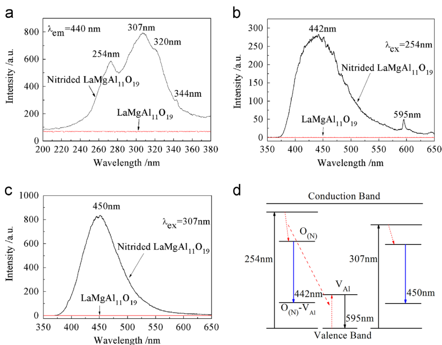
Fig. 5. Photoluminescence spectra of the as-prepared LaMgAl_{11}O_{19} and nitrided LaMgAl_{11}O_{19} phosphors. (a) Excitation spectrum ( \lambda_{em}=440 nm), (b) emission spectrum ( \lambda_{ex}=254 nm), (c) emission spectrum ( \lambda_{ex}=307 nm), and (d) energy level transition diagram.
