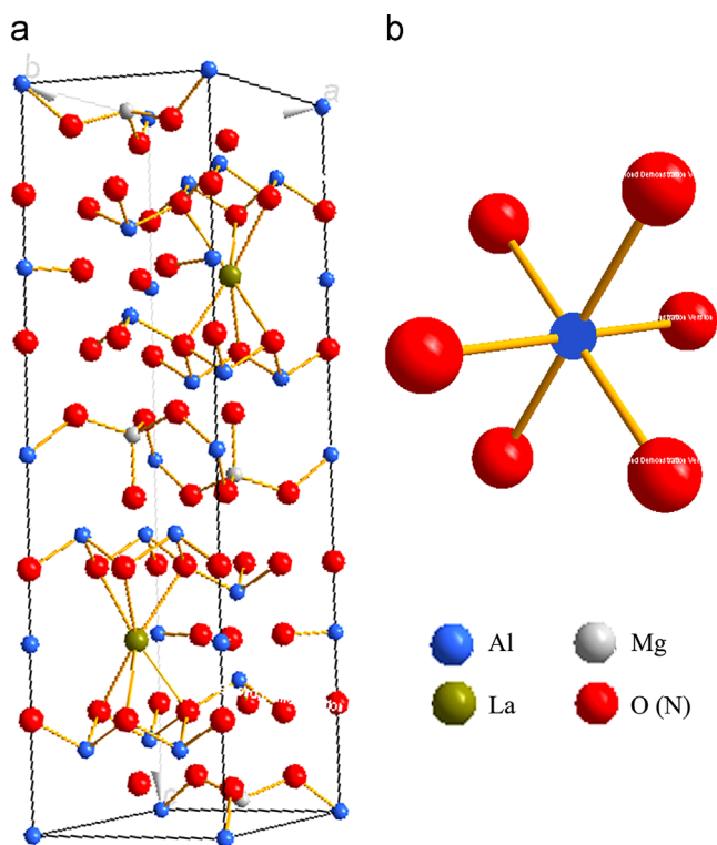
Fig. 3. Crystal structures of nitrided \text{LaMgAl}_{11}\text{O}_{19} . (a) The unit cell structure of nitrided \text{LaMgAl}_{11}\text{O}_{19} and (b) the coordination environment of Al.
