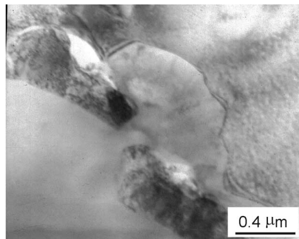
Fig. 3. Bright-field electron micrograph showing the early stage grain boundary migration between two pinning MgO precipitates in \text{ZrO}_2 stabilized with 11 mol% MgO.
