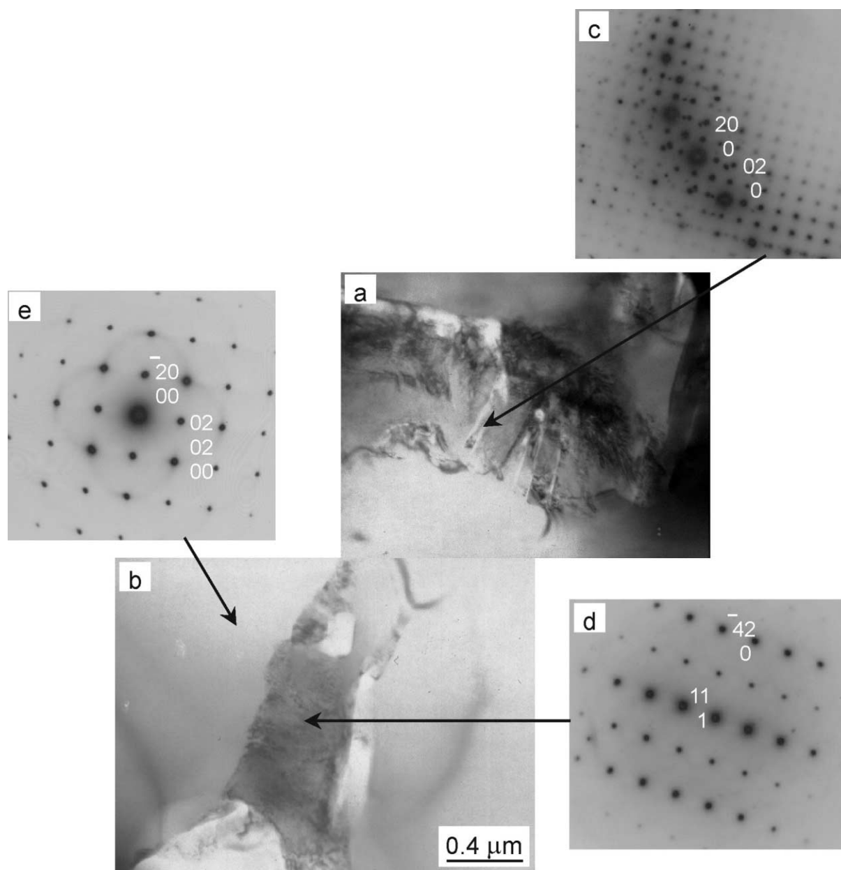
Fig. 6. Bright field electron micrographs of the transformed area at the grain boundaries of \text{ZrO}_2 stabilized with 11 mol% MgO showing (a) monoclinic phase of \text{ZrO}_2 together with MgO rods; and (b) tetragonal \text{ZrO}_2 phase with MgO precipitates and cubic \text{ZrO}_2 surrounding grains. The selected area diffraction patterns taken at: (c) zone axis [00\bar{1}] of m- \text{ZrO}_2 , (d) zone axis [1\bar{2}\bar{3}] of t- \text{ZrO}_2 and (e) zone axis [001] of c- \text{ZrO}_2 .
