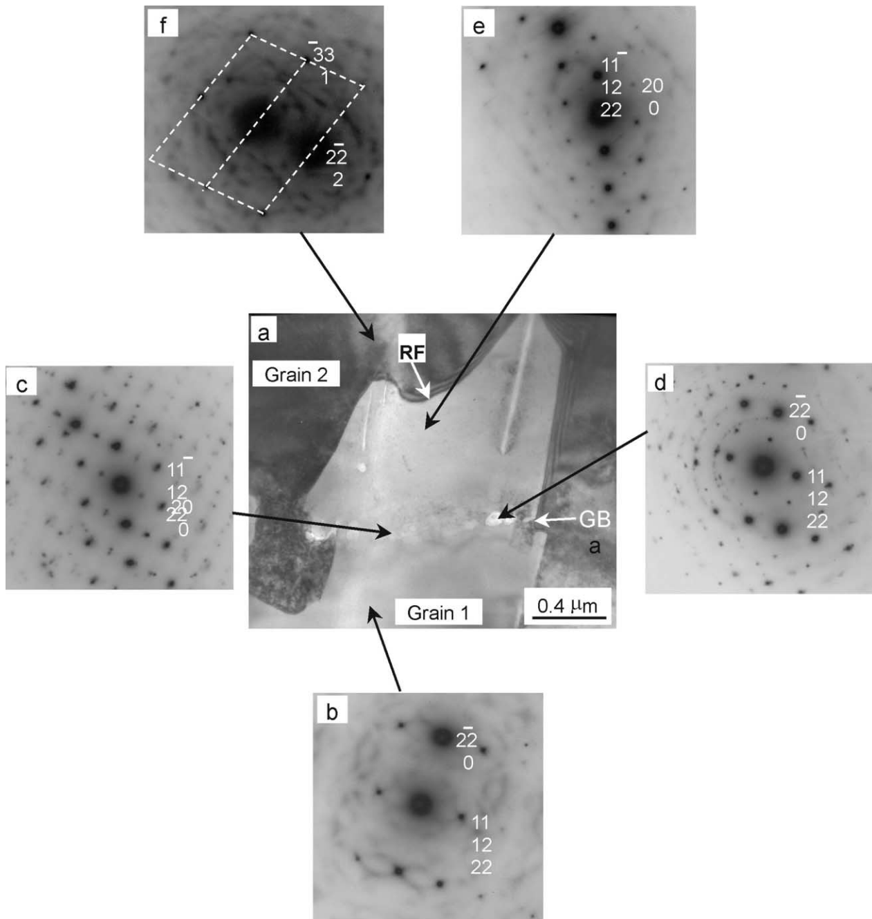
Fig. 4. Bright-field electron micrograph showing grain boundary zone decomposed by the grain boundary diffusion in ZrO 2 stabilized with 8 mol% MgO. (a) Selected area diffraction patterns taken from different areas marked by arrows: (b) zone axis [11\bar{2}] of c-ZrO 2 , (c) zone axis [011] of m-ZrO 2 , (d) zone axis [11\bar{2}] of m-ZrO 2 , (e) zone axis [011] of m-ZrO 2 and (f) zone axis [1\bar{2}\bar{3}] of c-ZrO 2 . GB, original grain boundary; RF, reaction front.
